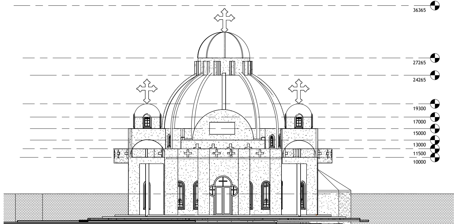
South Elevation
