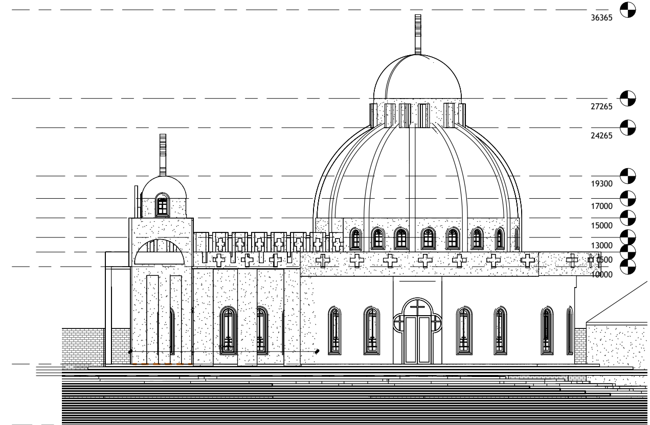
EastElevation
