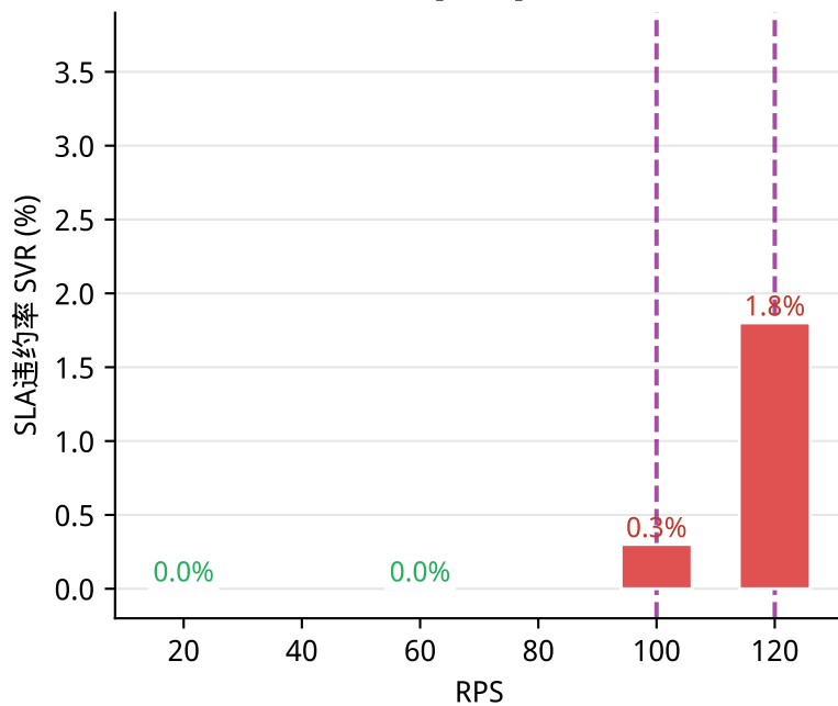
(A) SLA违约率 vs RPS [实测]
