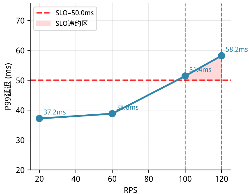
(B) P99延迟 vs RPS [实测]
