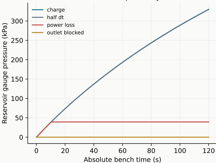
Fan coasts after power loss at 10 s
