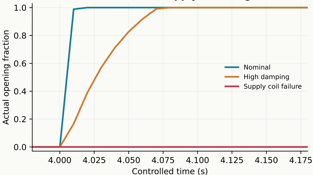
Coil failure does not stop the vehicle
