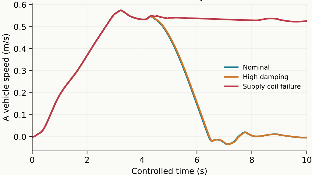
Coil failure does not stop the vehicle
