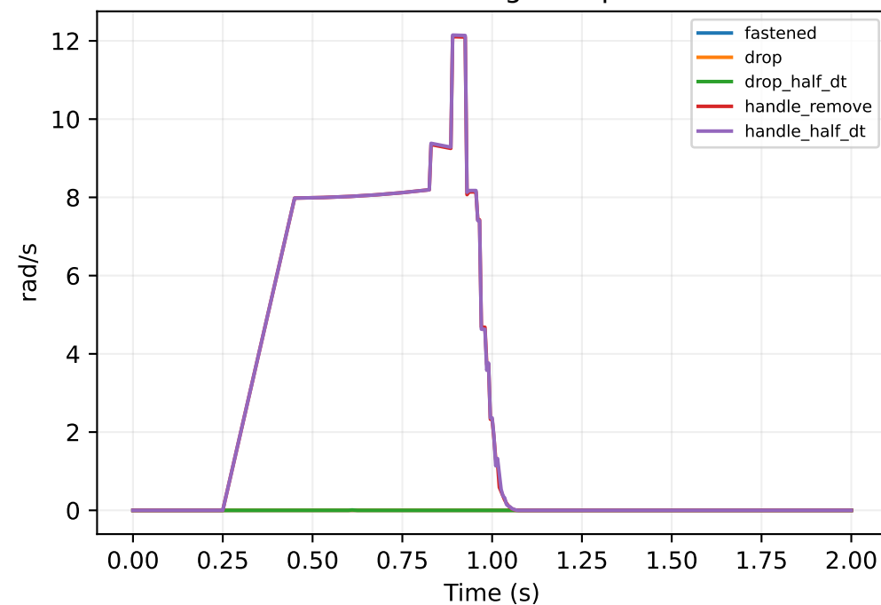
First cover angular speed
