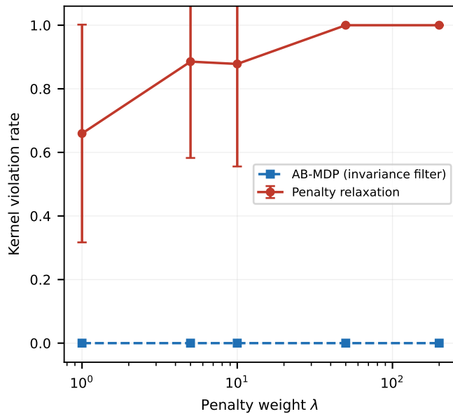
(d) Violation vs. penalty weight (8 seeds x 800 episodes; \tilde{R} = 2 )
