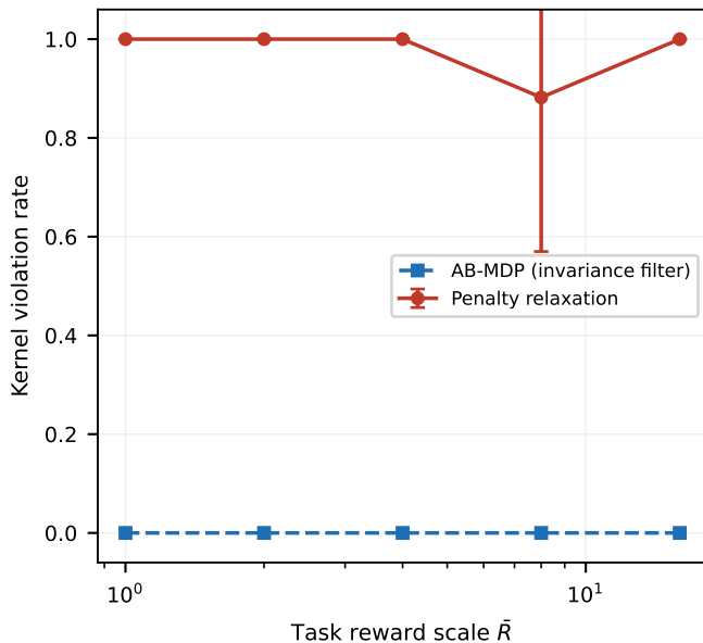
(c) Violation vs. reward scale (8 seeds x 800 episodes)
