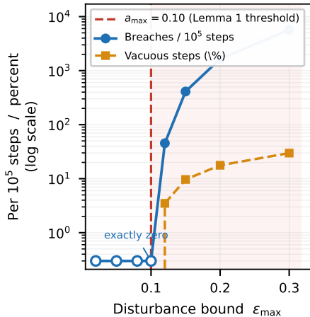
(c) Does the kernel erode where Lemma 1 says? (8 seeds \times 800 episodes)
