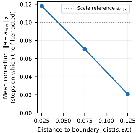
(b) Size of the corrective action
