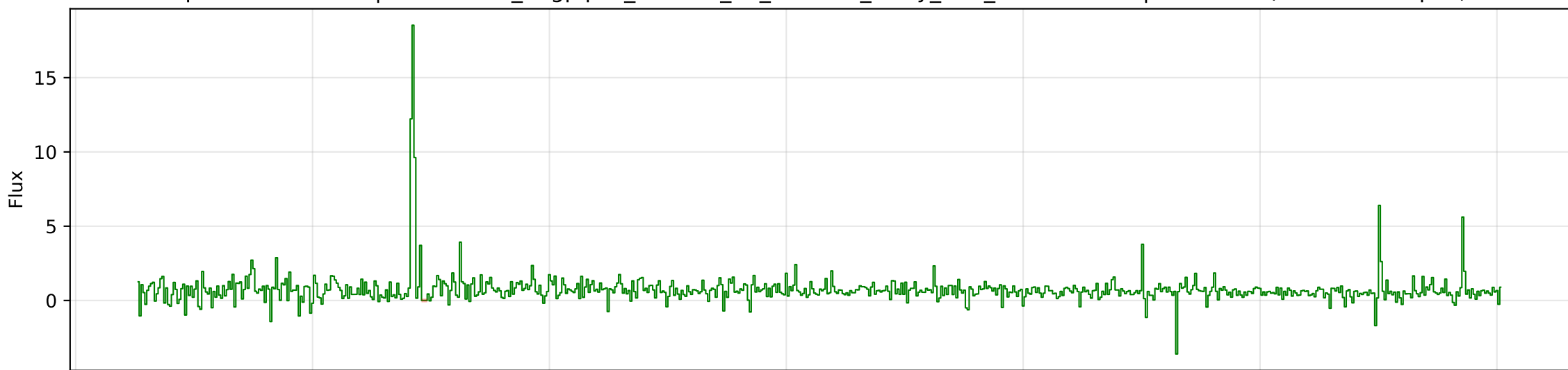
Split: VALIDATION | ID: cosmos_bagpipes_519784_2h_z1.4959_noisy_deZ_rebinned.fits | z: 1.4959 (normalized spec)
