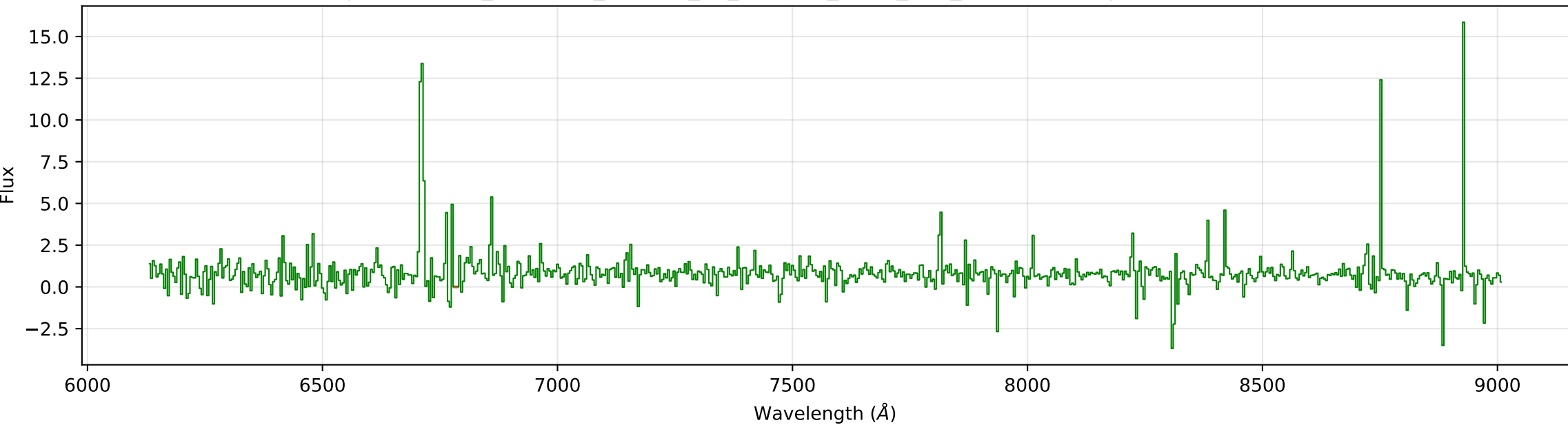
Split: TEST | ID: cosmos_bagpipes_301545_2h_z1.4787_noisy_deZ_rebinned.fits | z: 1.4787 (normalized spec)
