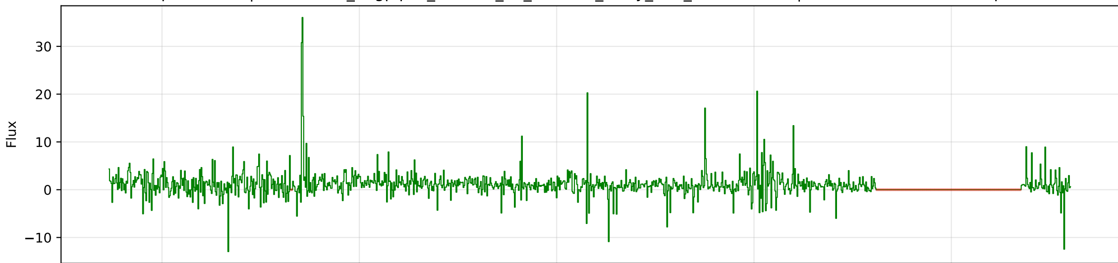
Split: VALIDATION | ID: cosmos_bagpipes_293804_2h_z1.1721_noisy_deZ_rebinned.fits | z: 1.1721 (normalized spec)
