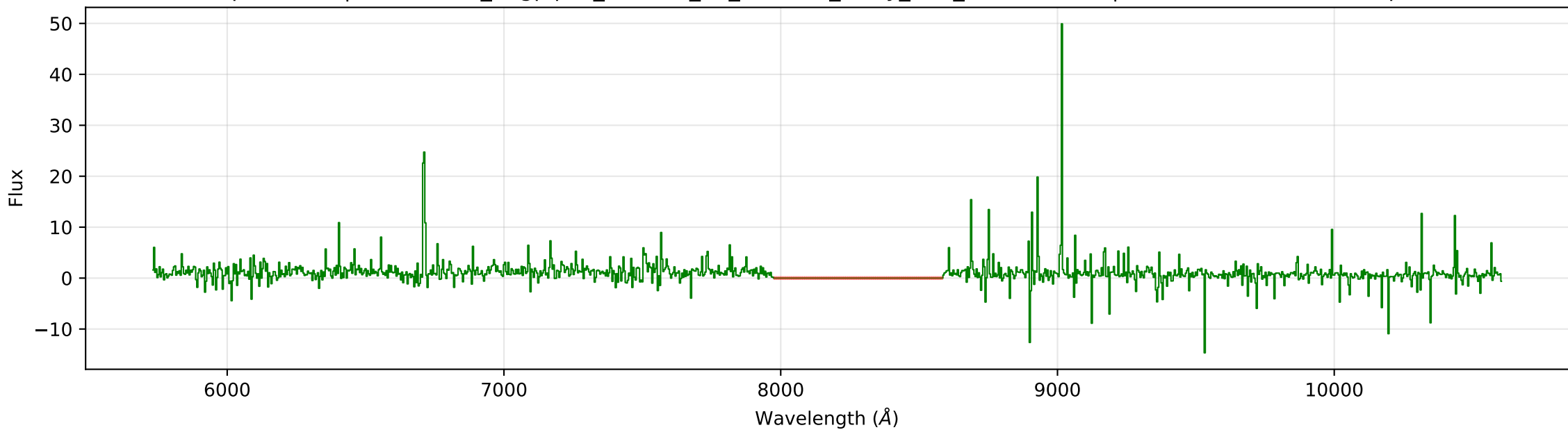
Split: TEST | ID: cosmos_bagpipes_203971_2h_z2.0461_noisy_deZ_rebinned.fits | z: 2.0461 (normalized spec)
