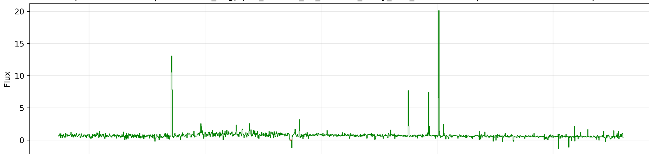
Split: VALIDATION | ID: cosmos_bagpipes_293804_2h_z1.1721_noisy_deZ_rebinned.fits | z: 1.1721 (normalized spec)
