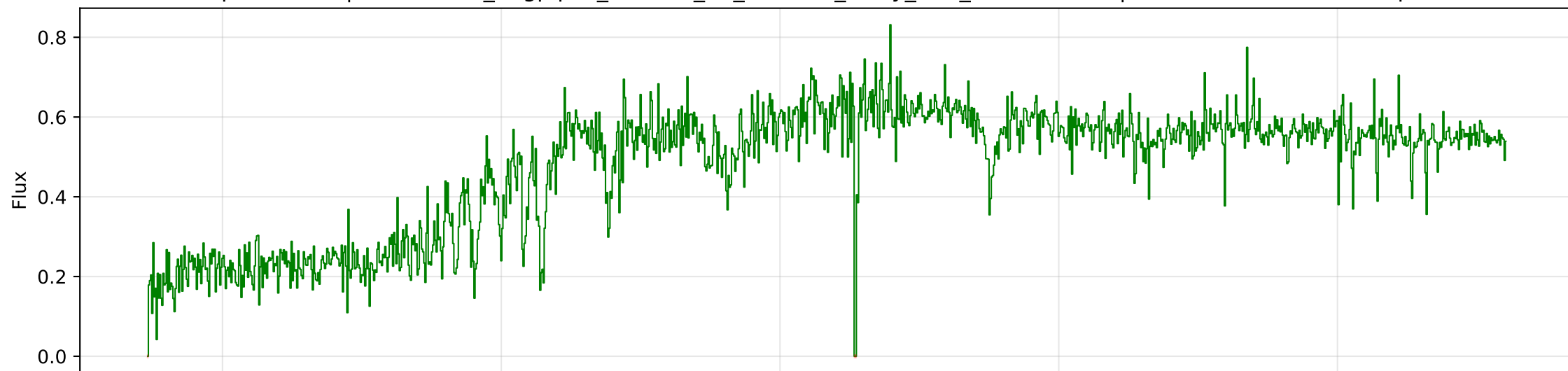
Split: TRAIN | ID: cosmos_bagpipes_203188_8h_z1.0330_noisy_deZ_rebinned.fits | z: 1.0330 (normalized spec)
