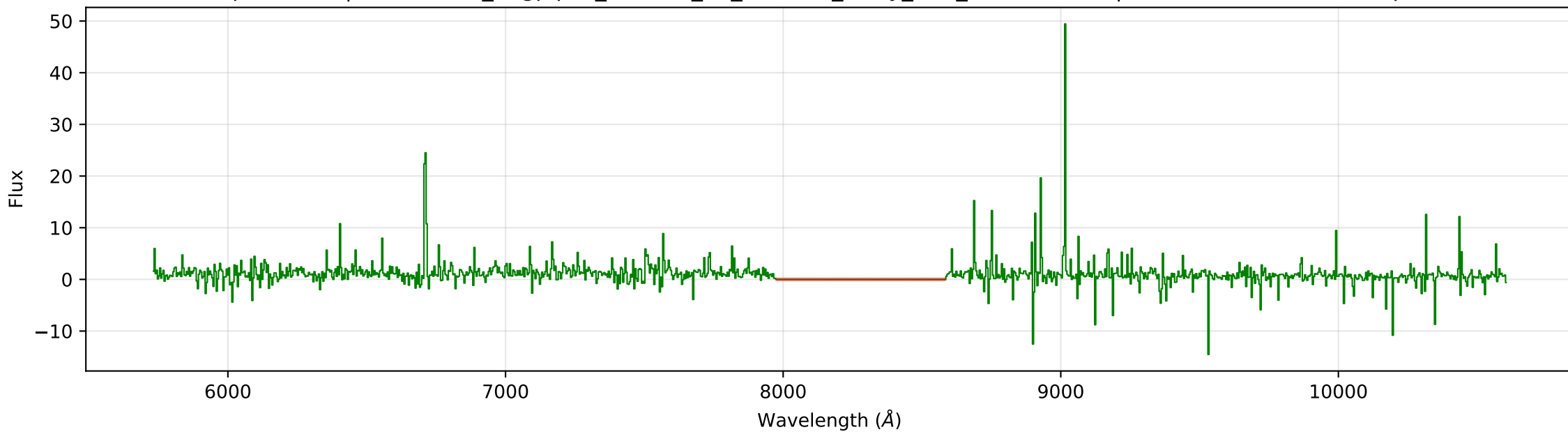
Split: TEST | ID: cosmos_bagpipes_203971_2h_z2.0461_noisy_deZ_rebinned.fits | z: 2.0461 (normalized spec)
