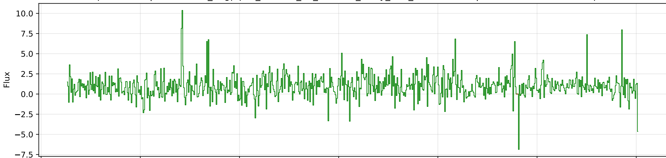
Split: VALIDATION | ID: cosmos_bagpipes_770660_2h_z2.1303_noisy_deZ_rebinned.fits | z: 2.1303 (normalized spec)
