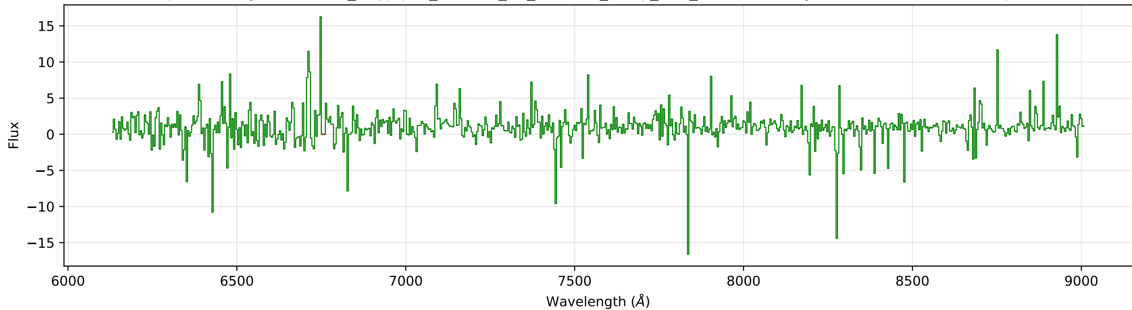
Split: TEST | ID: cosmos_bagpipes_459385_2h_z1.4891_noisy_deZ_rebinned.fits | z: 1.4891 (normalized spec)
