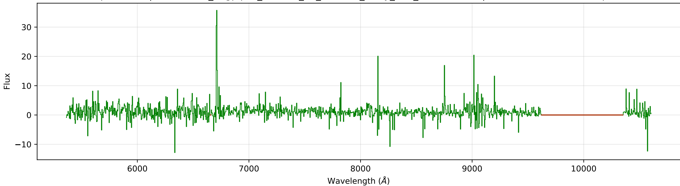
Split: TEST | ID: cosmos_bagpipes_328590_2h_z1.5260_noisy_deZ_rebinned.fits | z: 1.5260 (normalized spec)
