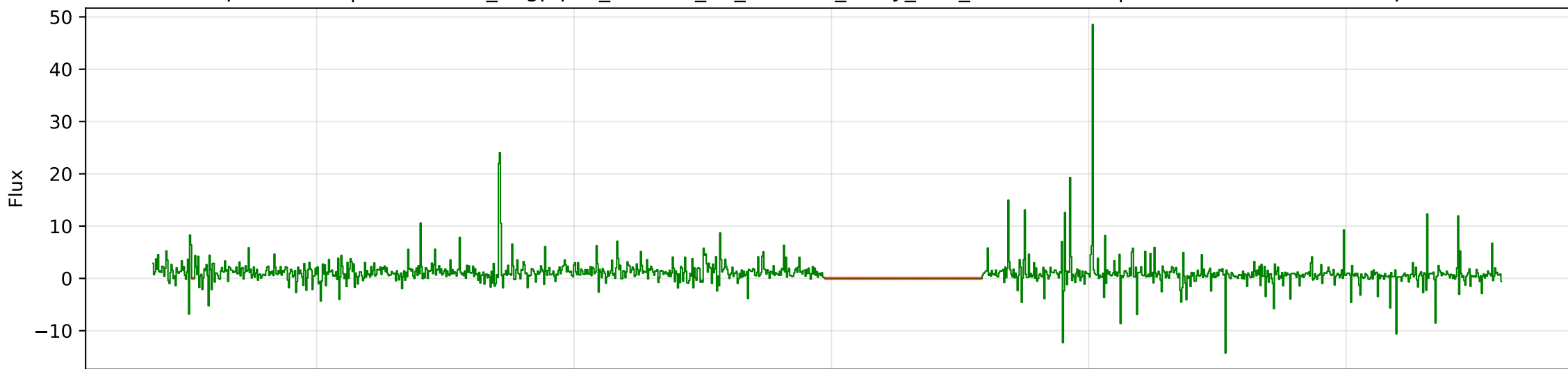
Split: VALIDATION | ID: cosmos_bagpipes_248408_2h_z2.0560_noisy_deZ_rebinned.fits | z: 2.0560 (normalized spec)
