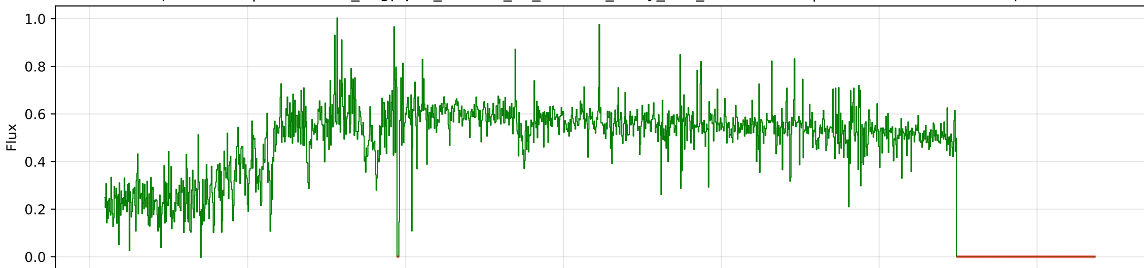
Split: TRAIN | ID: cosmos_bagpipes_208383_8h_z1.1144_noisy_deZ_rebinned.fits | z: 1.1144 (normalized spec)
