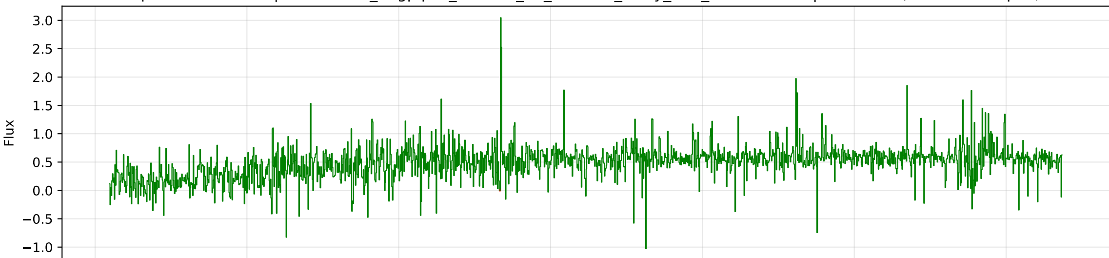
Split: VALIDATION | ID: cosmos_bagpipes_214956_8h_z0.9403_noisy_deZ_rebinned.fits | z: 0.9403 (normalized spec)
