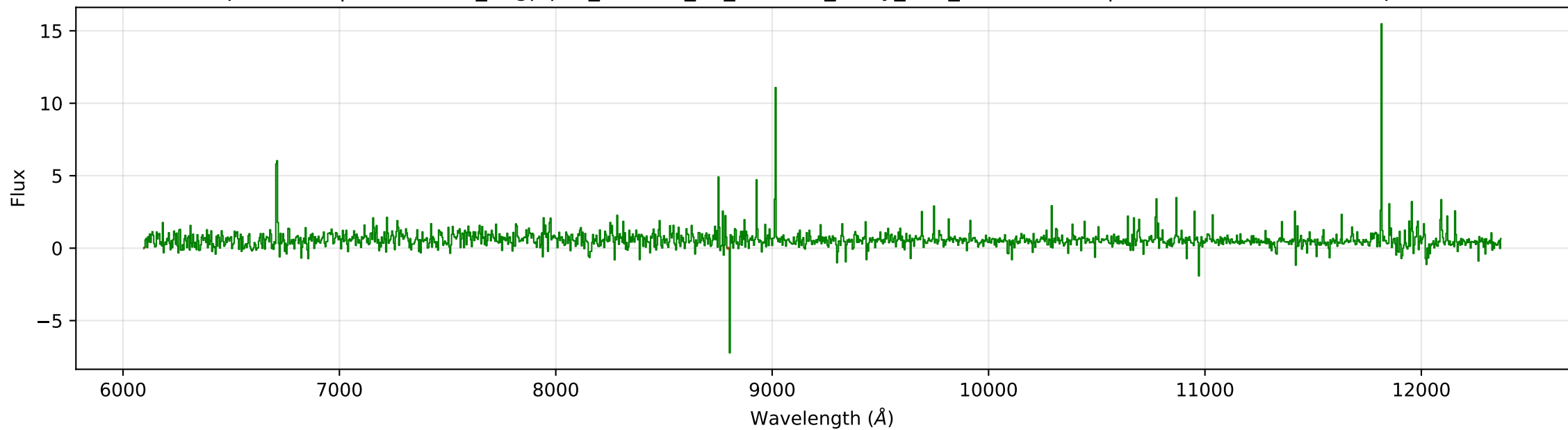
Split: TEST | ID: cosmos_bagpipes_204478_2h_z0.9116_noisy_deZ_rebinned.fits | z: 0.9116 (normalized spec)
