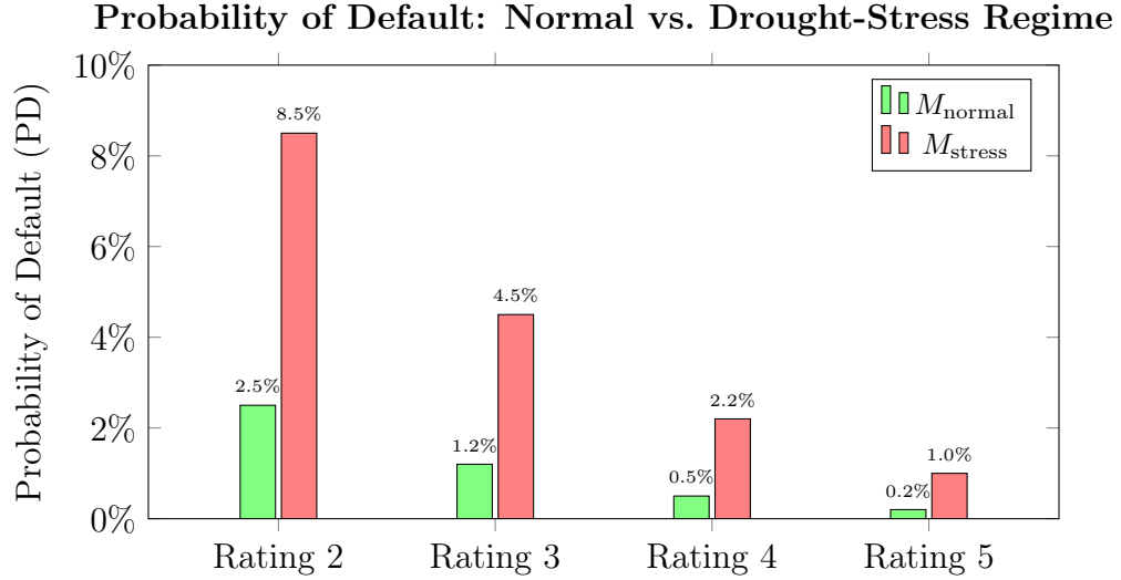
Figure 6: One-quarter Probability of Default by credit rating under the Normal and Drought-Stress regimes. Default probabilities increase by a factor of 3–5× during drought conditions.
