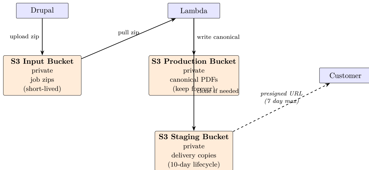
Figure 3: Three-bucket storage model. Input bucket holds job payloads. Production bucket keeps the canonical PDF forever. Staging bucket receives a copy only when large-file delivery via presigned URL is required; objects auto-expire after 10 days, presigned URLs valid for max 7 days — URL always expires before the underlying object.
