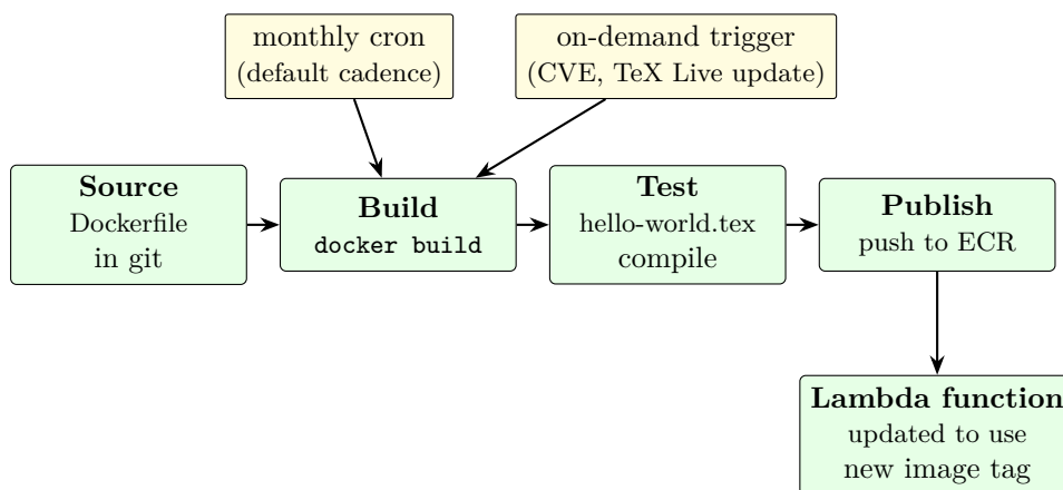
Figure 4: ECR-container Image Builder pipeline for the Lambda LaTeX image. Monthly cadence by default; on-demand trigger for CVE response or toolchain updates. Symmetric with existing nginx/php83 AMI pipelines — reuses operational patterns.
