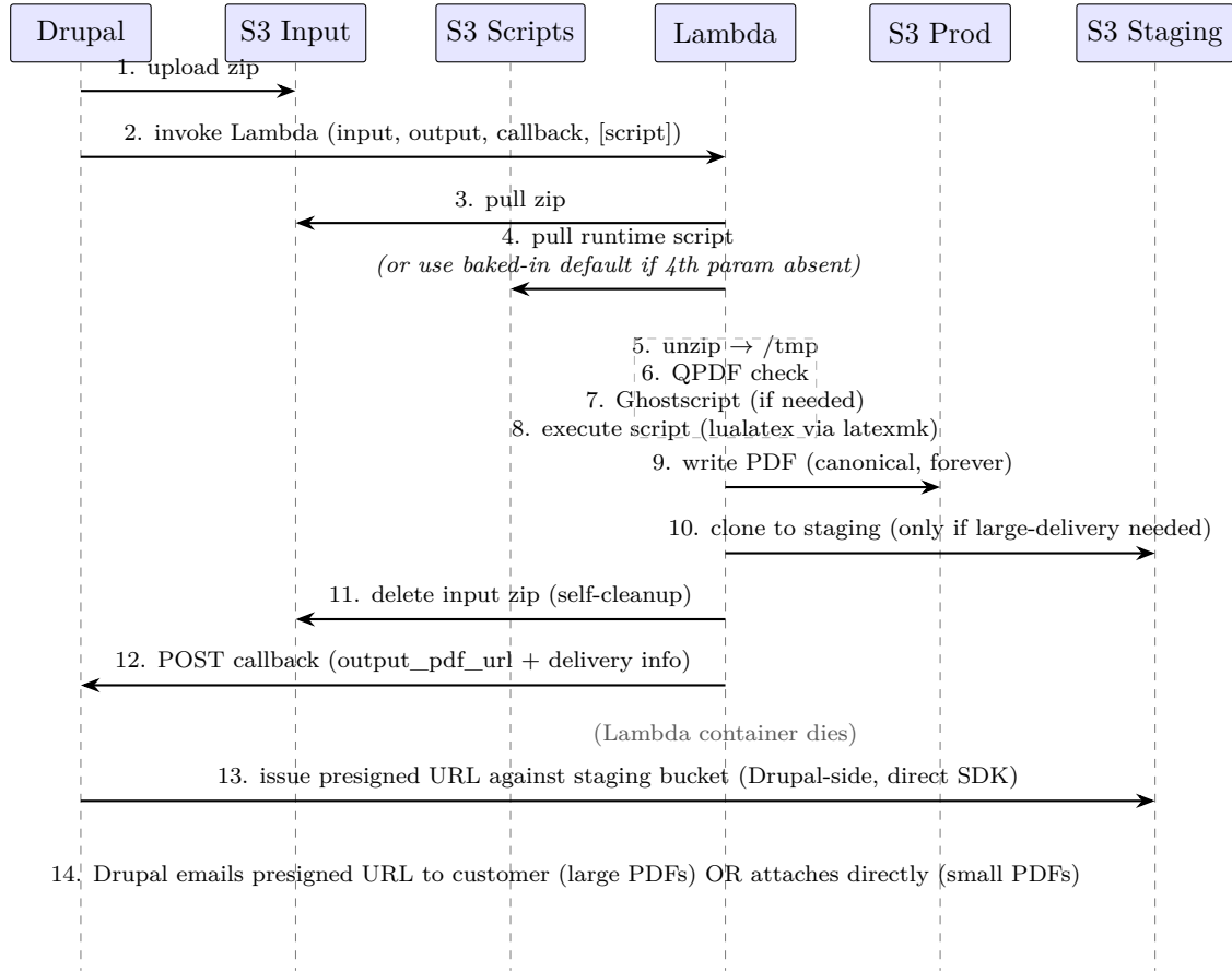
Figure 1: End-to-end sequence: Drupal → Lambda → dual-write to production + staging → callback → time-limited customer delivery. Step 4 fetches the runtime script when the optional 4th parameter is provided; otherwise Lambda uses the script baked into the container image.
