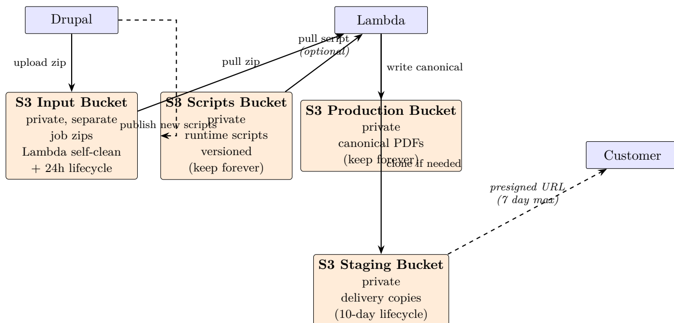
Figure 3: Four-bucket storage model. Input holds job payloads (short-lived). Scripts holds runtime scripts that Lambda can optionally pull for per-invocation flexibility (long-lived, versioned by convention). Production keeps the canonical PDF forever. Staging receives a copy only when large-file delivery via presigned URL is required; objects auto-expire after 10 days, presigned URLs valid for max 7 days — URL always expires before the underlying object. Scripts kept in a separate bucket so its long-lived nature doesn't pollute the short-lived buckets and vice versa.
