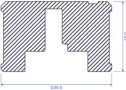
KNOB - SECTION THROUGH THE D-FLAT 2:1 (printed top face down, i.e. upside down from this view)
