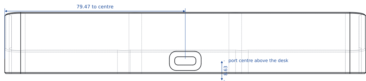
BACK VIEW (looking at the USB port)
