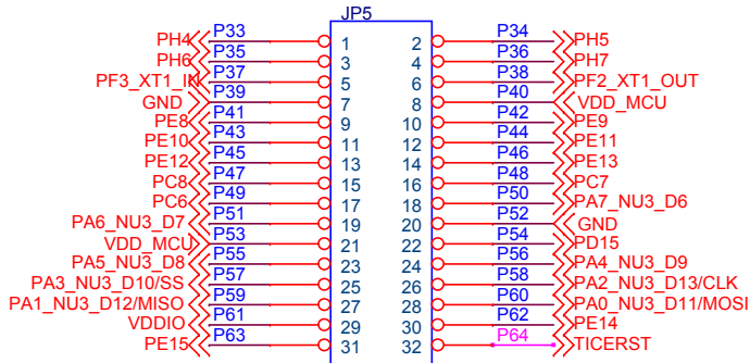
HEADER 2.54 16X2 male
