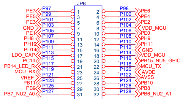
HEADER 2.54 16X2 male
