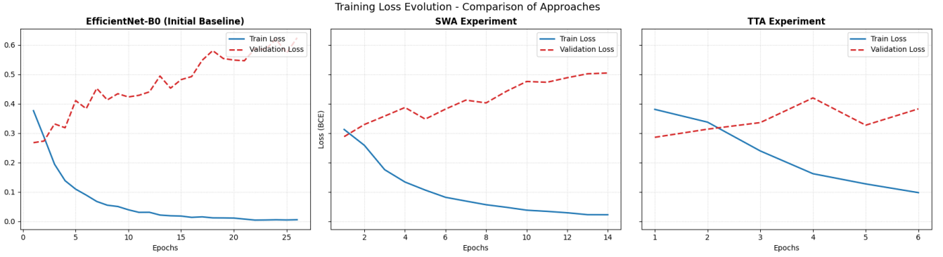
FIGURE 5 Baseline model training evolution curve.
