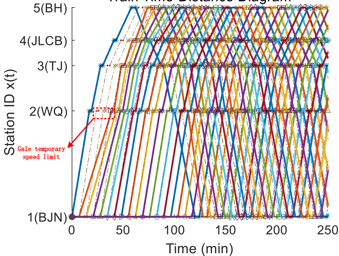
Train Time-Distance Diagram
