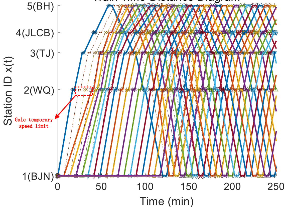
Train Time-Distance Diagram
