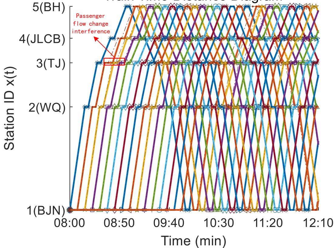
Train Time-Distance Diagram
