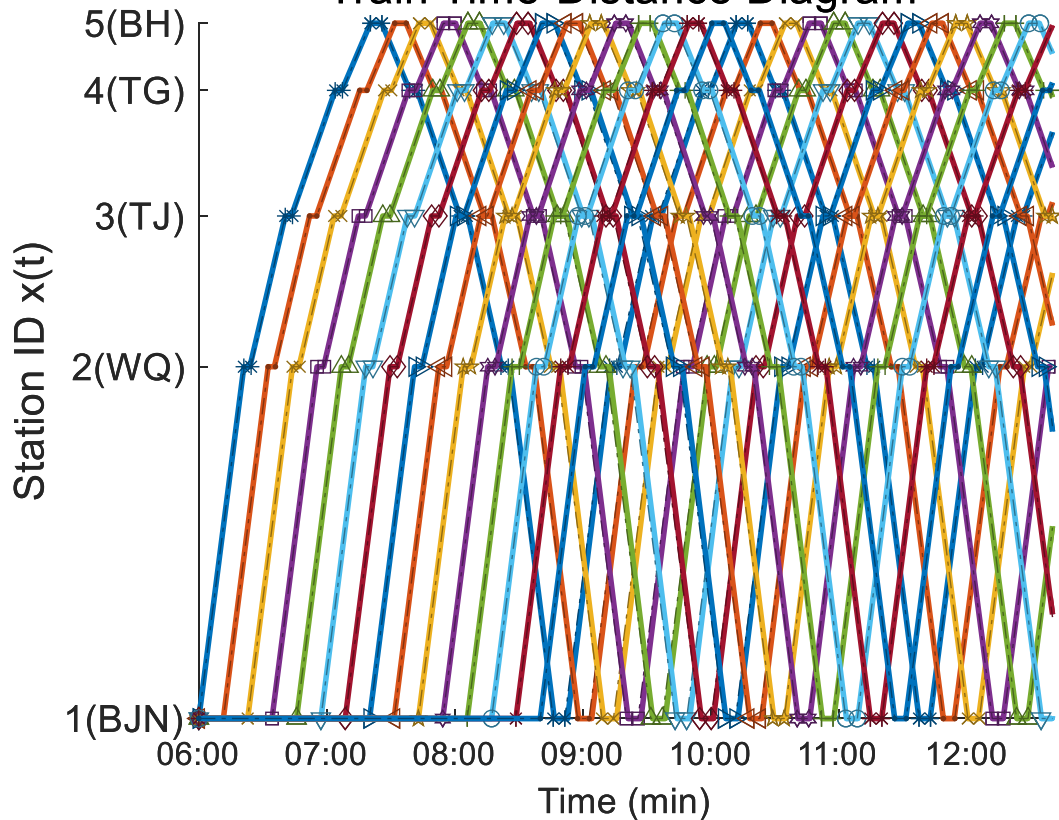
Train Time-Distance Diagram
