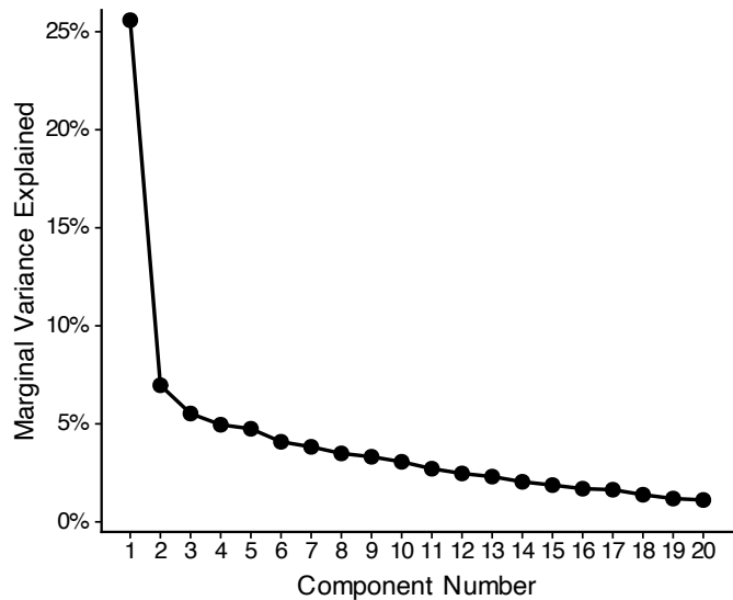
Scree Plot - Correctness Logistic PCA
