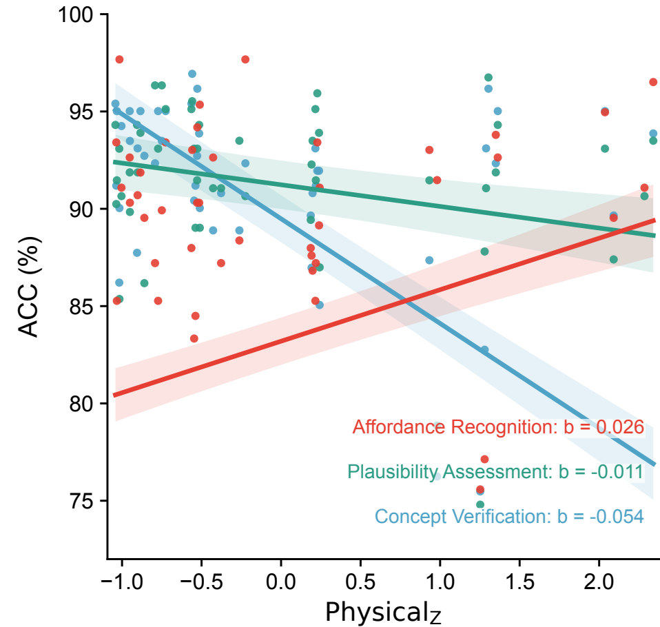
Physical z effect on ACC
