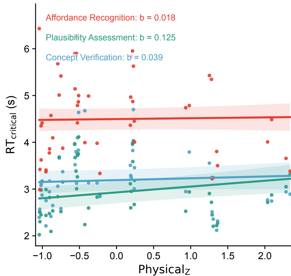
Physical z effect on RT critical
