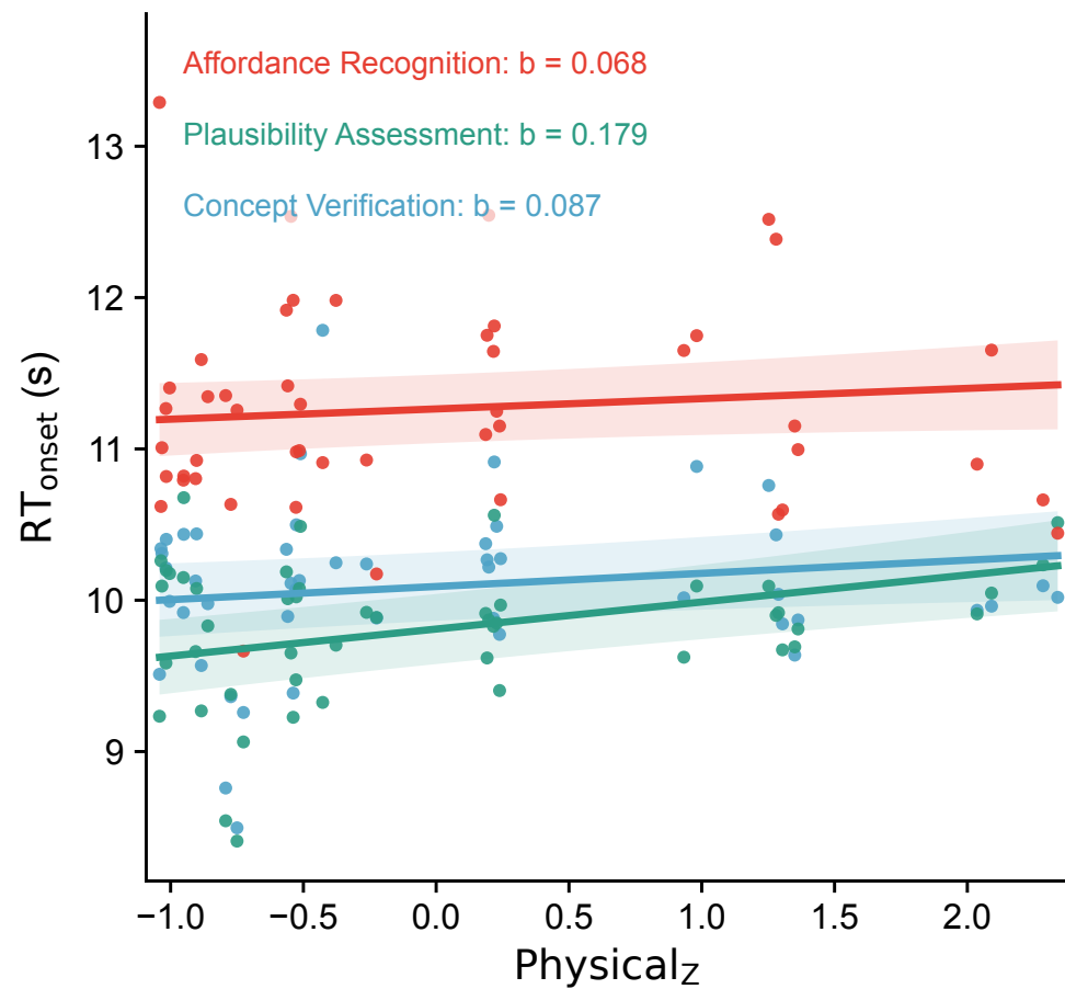
Physical z effect on RT onset
