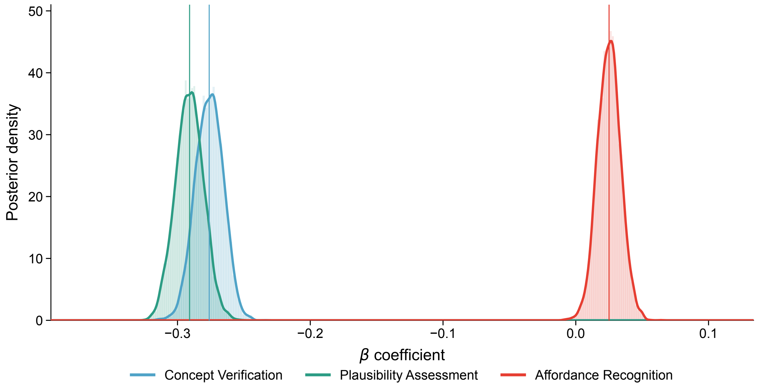
Model results: posterior distributions of v_{\text{Visual}_Z} coefficients
