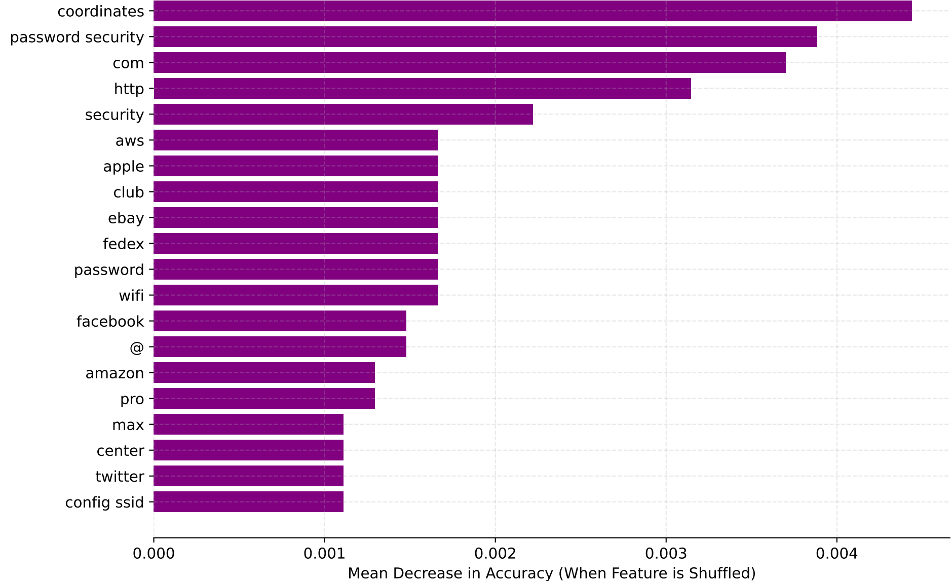
Top 20 Important N-grams (KNN) N-gram Range: (1, 2)
