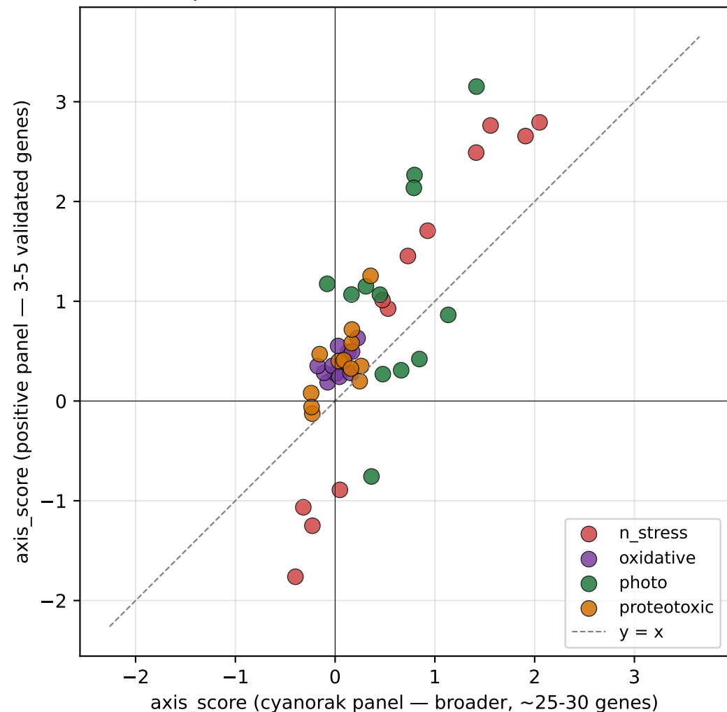
Sensitivity check: axis_score by panel kind (each point = one (axis, condition, omics, TP) cell)
