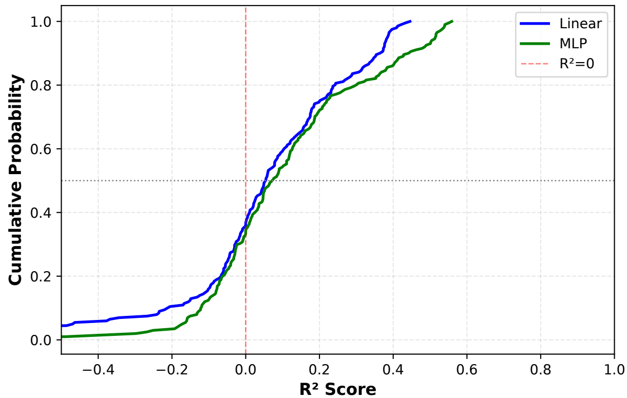
Cumulative Distribution of R^2 Scores
