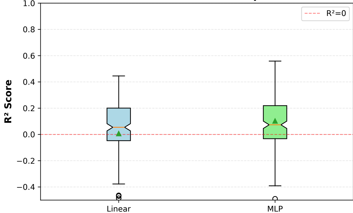
R^2 Score Distribution Comparison
