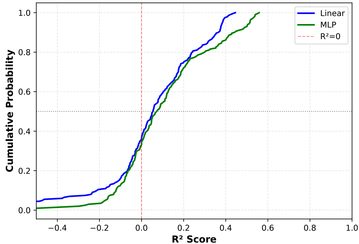
Cumulative Distribution of R^2 Scores
