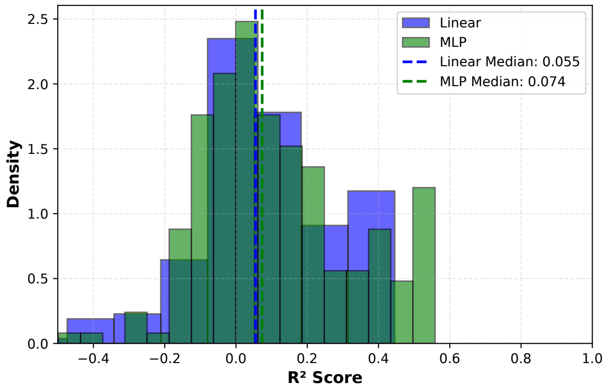
Distribution of R^2 Scores
