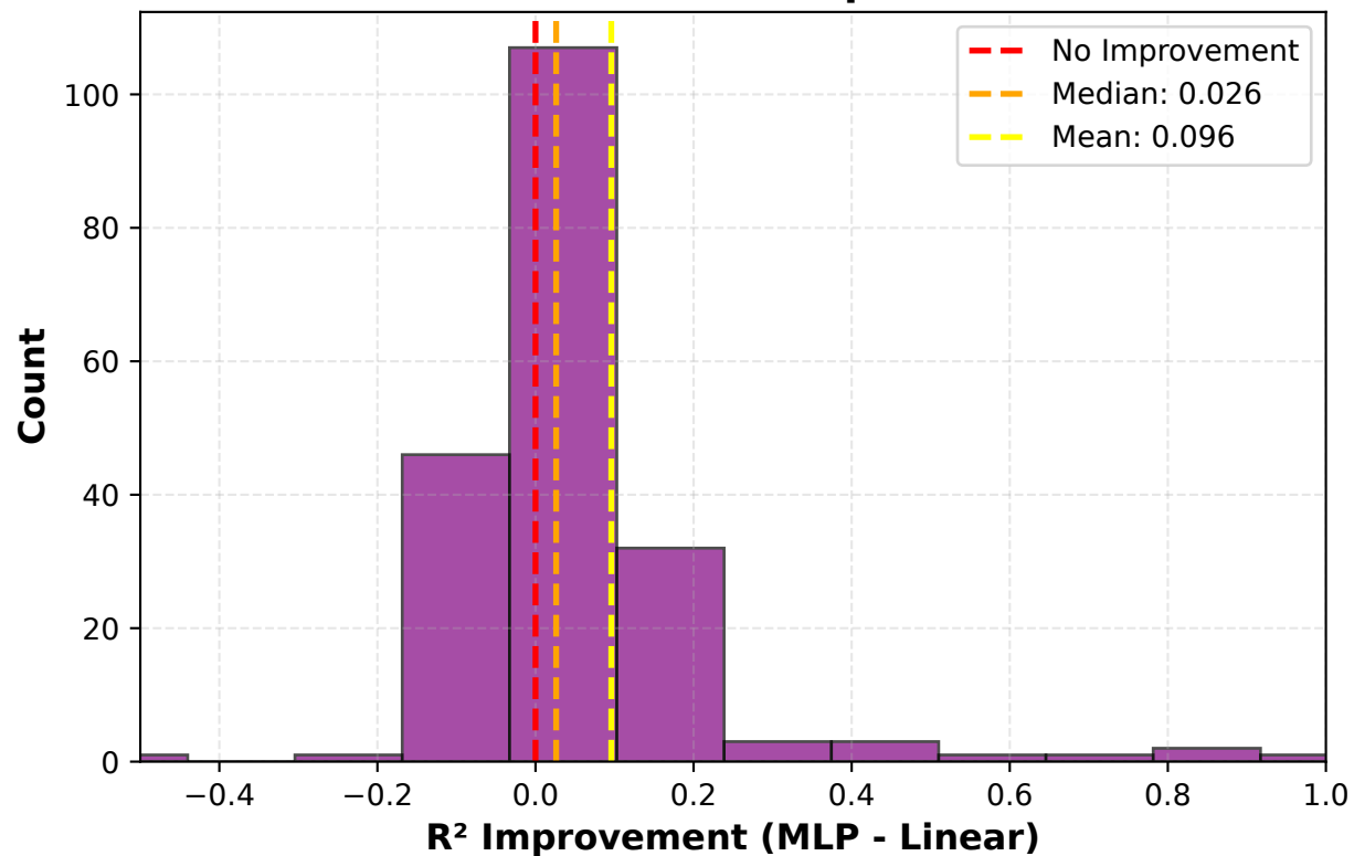
Distribution of R^2 Improvement
