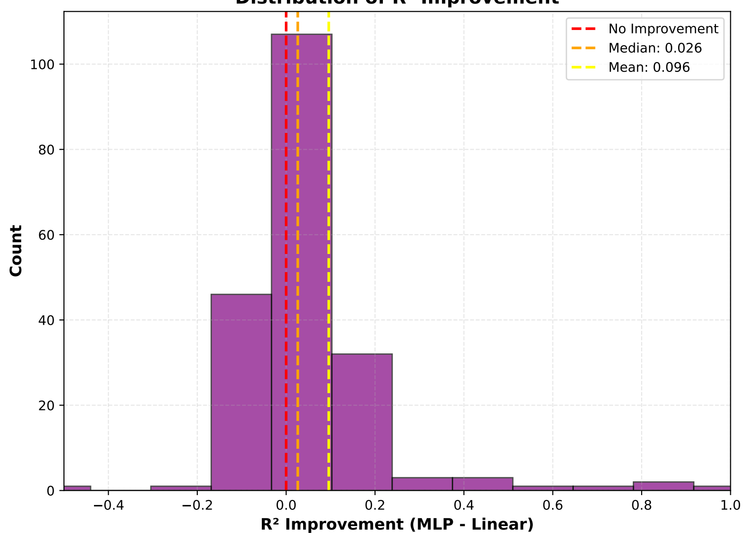
Distribution of R^2 Improvement
