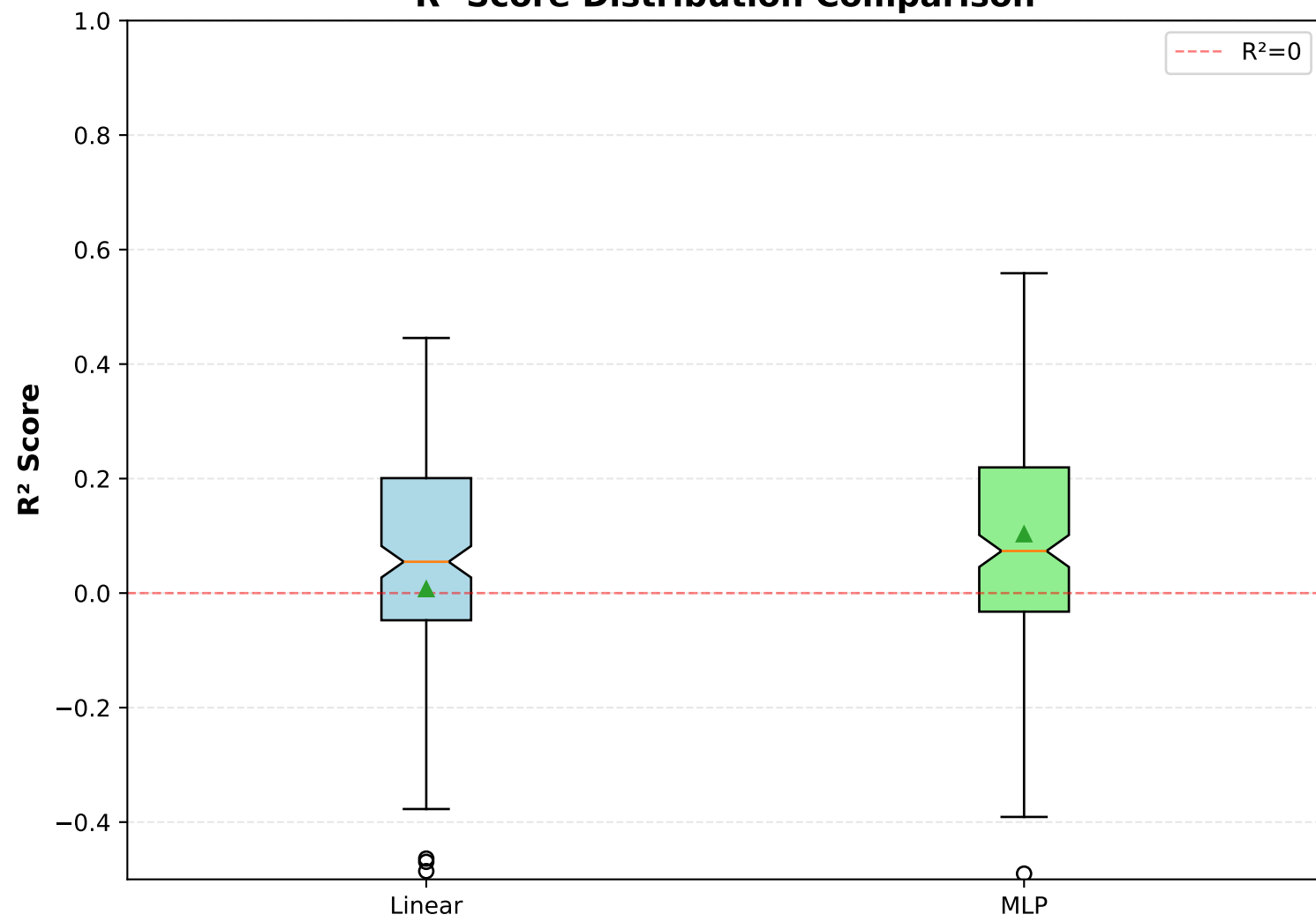
R^2 Score Distribution Comparison
