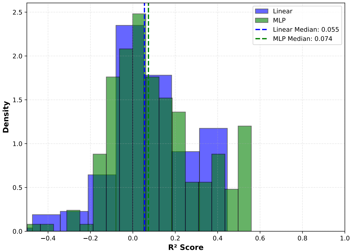
R^2 Score Distribution Comparison
