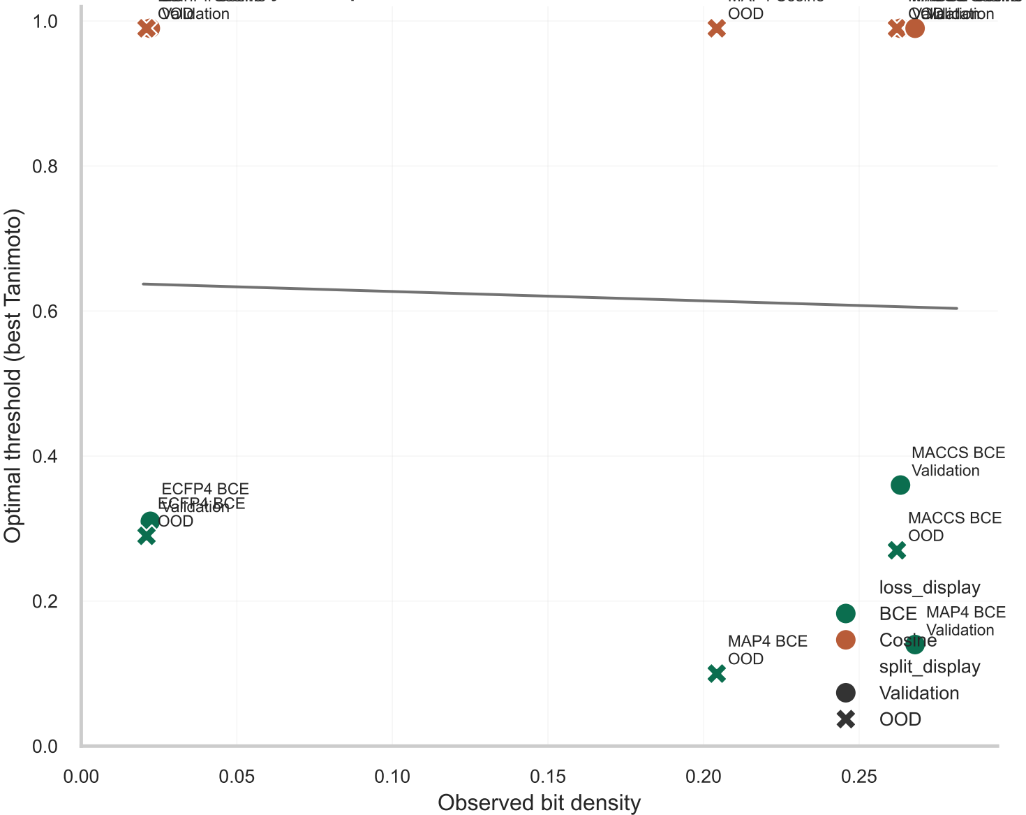
Bit Density vs Optimal Threshold Across Fine-tuned Conditions
