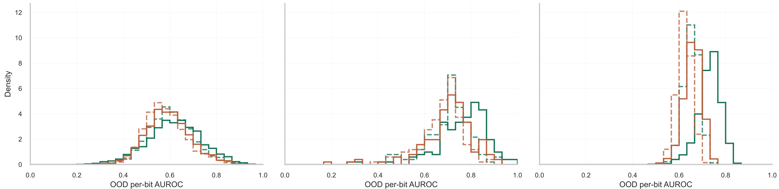
ECFP4
