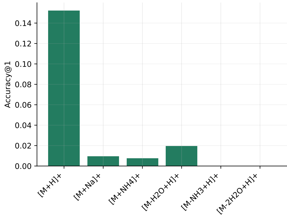
Adduct
