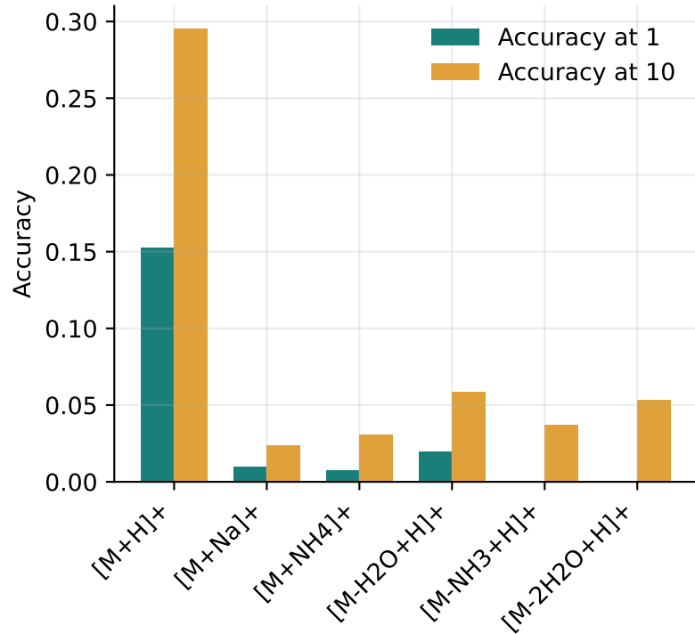
Adduct
