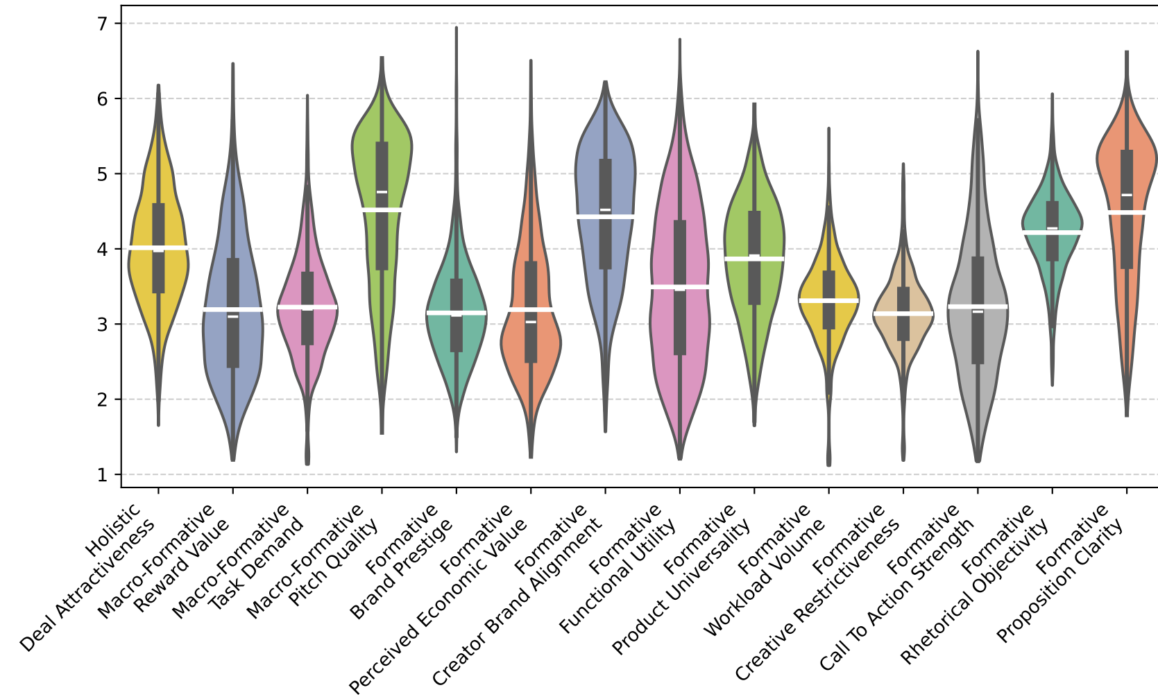
Model: Qwen 3.5
