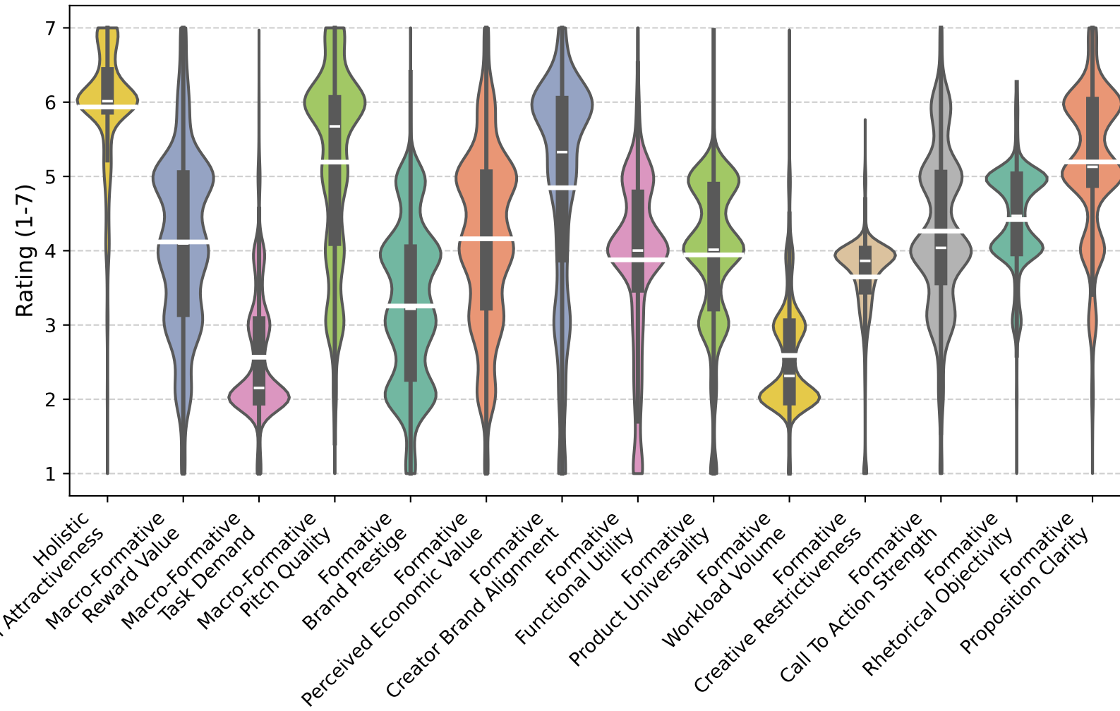
Model: Qwen 3
