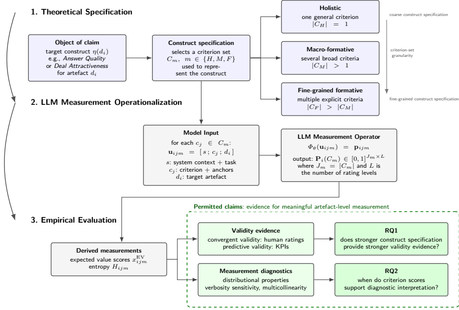
Fig. 3: Validity-guided framework for artefact-level LLM measurement. The framework proceeds from theoretical specification of the target construct \eta(d_i) , to LLM-based scoring of criteria c_j \in C_m , to empirical evaluation through validity evidence and measurement diagnostics. Here, m indexes the construct representation, C_m is its criterion set, and J_m = |C_m| is the number of criteria. For each artefact–criterion pair, the LLM returns a rating distribution \mathbf{p}_{ijm} , summarized by expected-value scores x_{ijm}^{\text{EV}} and entropy H_{ijm} . The informed holistic control used in the FeedbackQA analysis is omitted for simplicity because it functions as a design control rather than as a separate construct-representation category.
