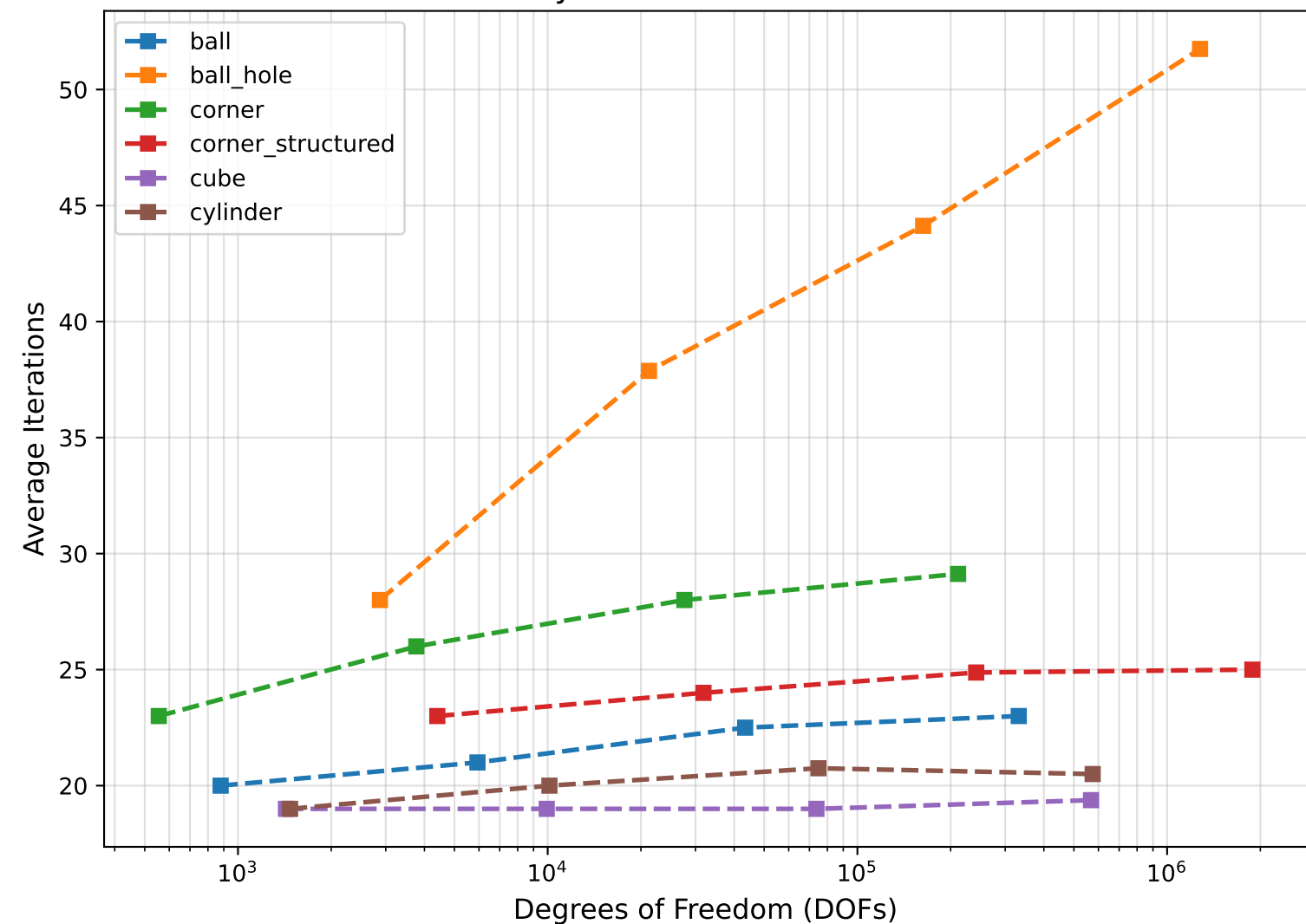
W-Cycle GMRES Iterations
