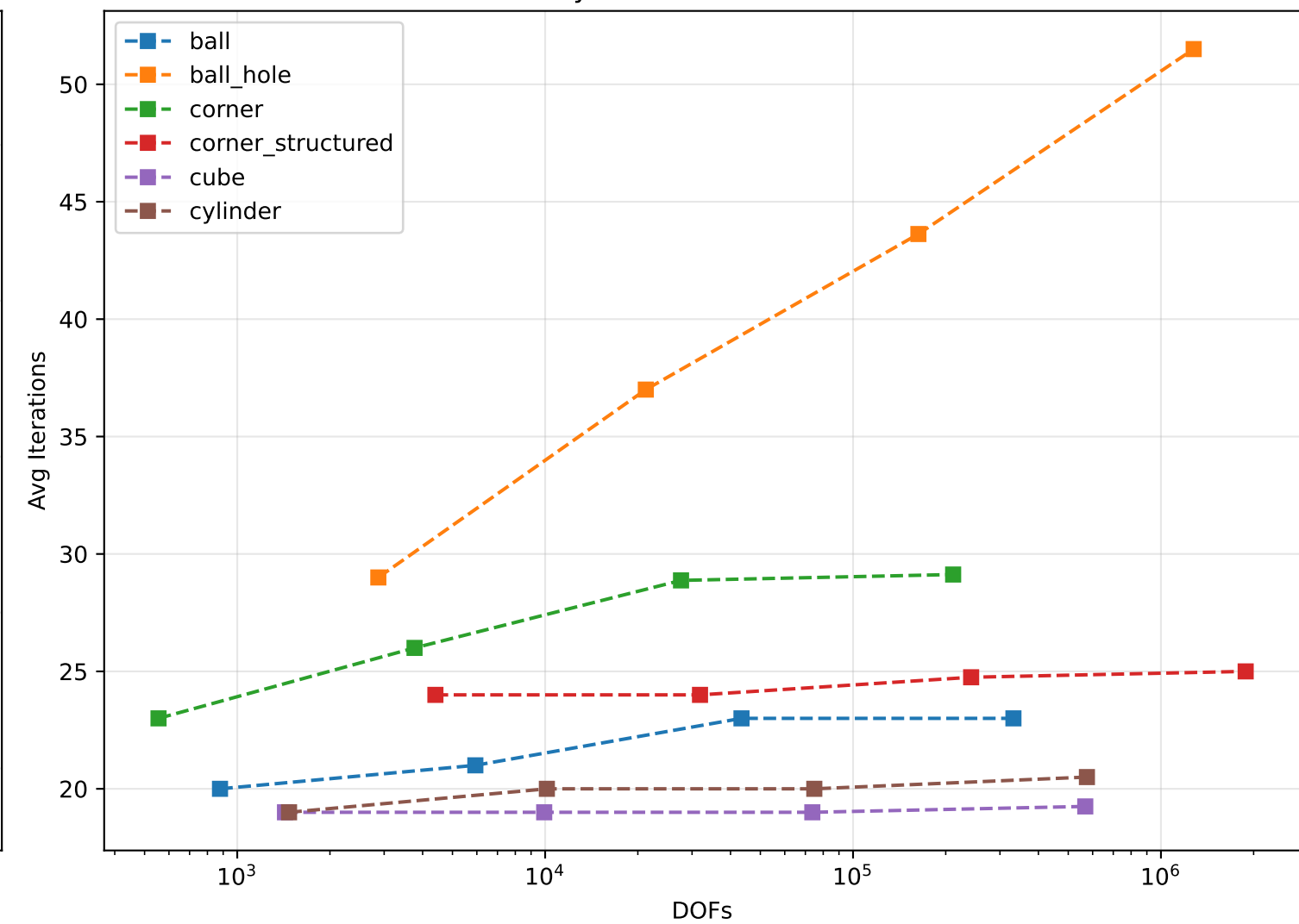
W-Cycle GMRES Iterations
