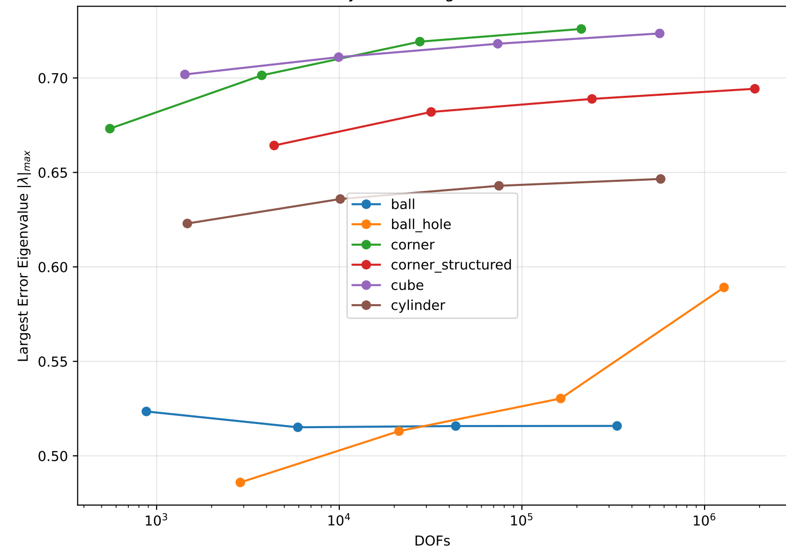
W-Cycle Convergence Factor
