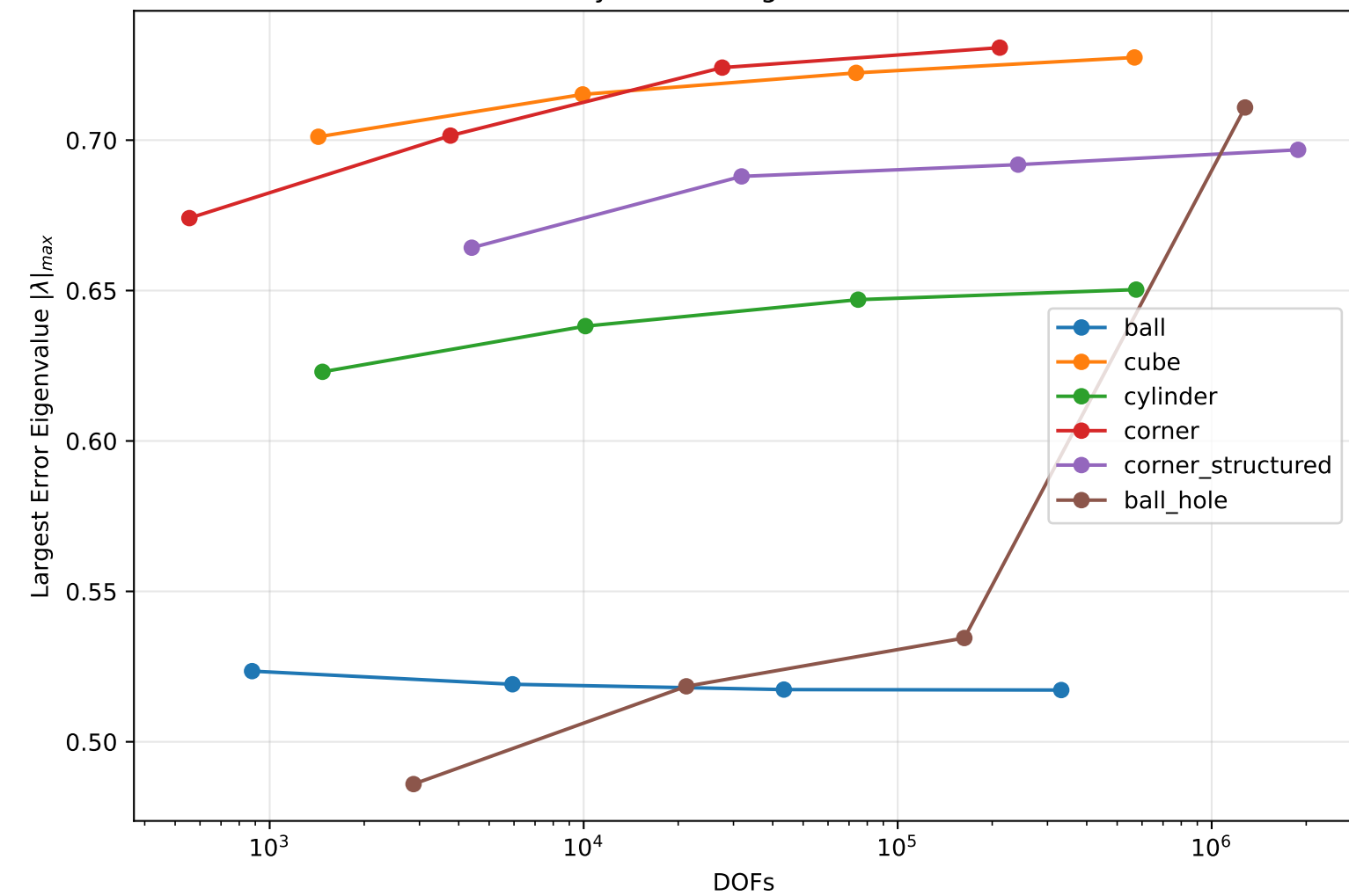
W-Cycle Convergence Factor
