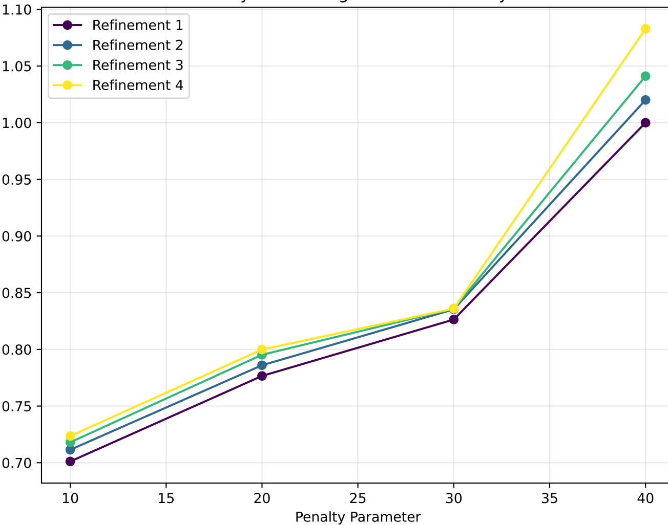
W-Cycle: Max Eigenvalue vs. Penalty
