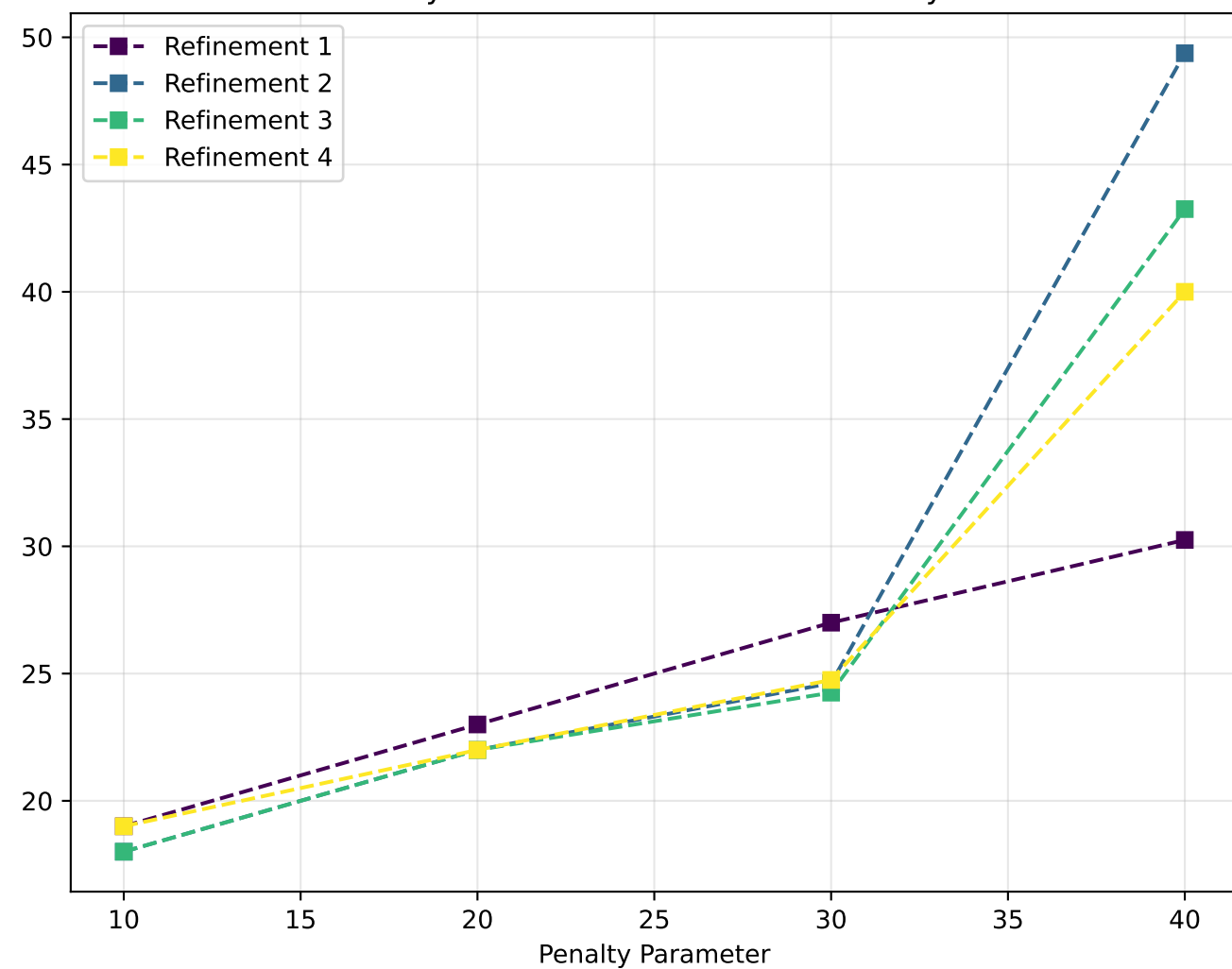
W-Cycle: GMRES Iterations vs. Penalty
