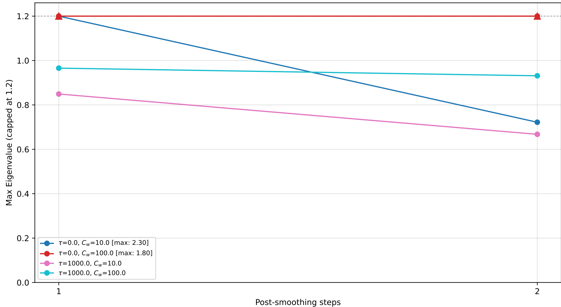
Post-smoothing vs Convergence (Mesh: corner.msh | V-Cycle) (Pre-smoothing fixed at 0, ref = 4)
