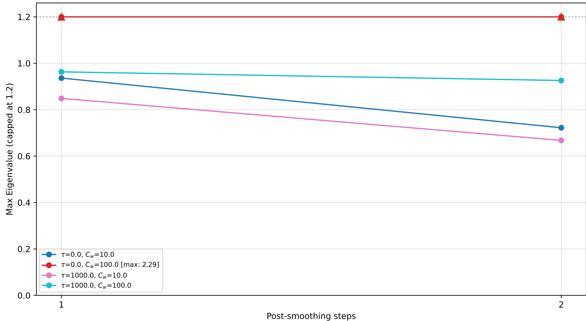
Post-smoothing vs Convergence (Mesh: cube.msh | V-Cycle) (Pre-smoothing fixed at 0, ref = 4)
