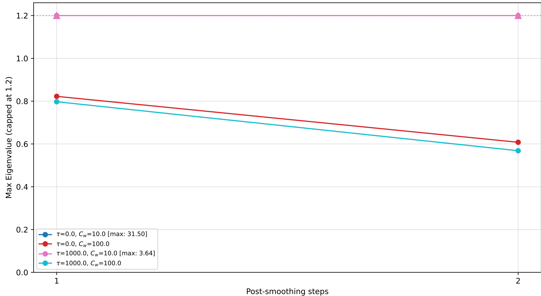
Post-smoothing vs Convergence (Mesh: cube_void.msh | V-Cycle) (Pre-smoothing fixed at 0, ref = 4)
