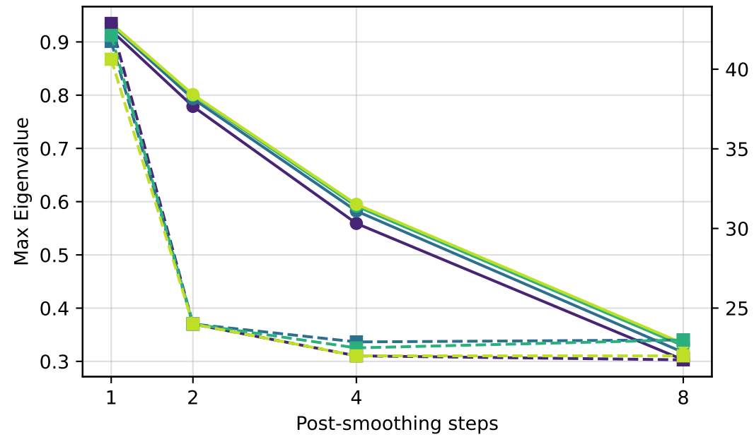
Penalty = 60.0
