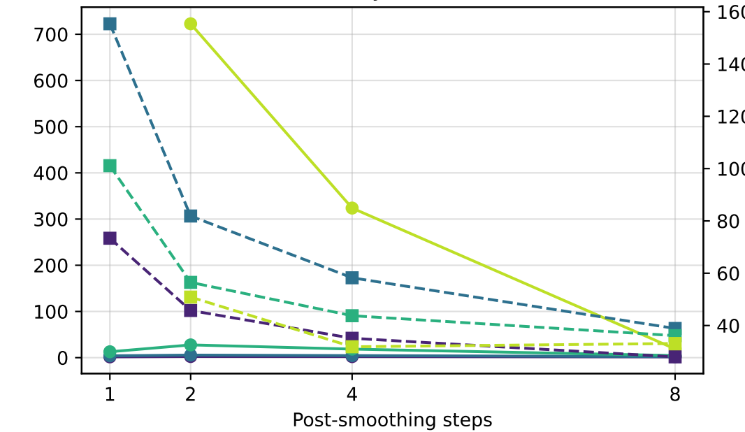
Penalty = 100.0
