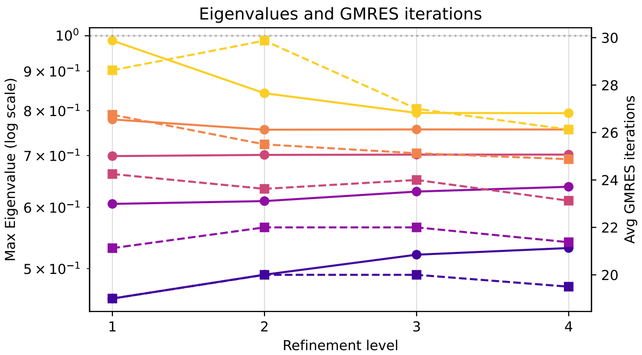
Penalty parameter and metric penalty=20.0 penalty=40.0 penalty=60.0 penalty=80.0 penalty=100.0 GMRES Eigenvalue
