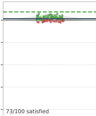
Multiagent Corridor
