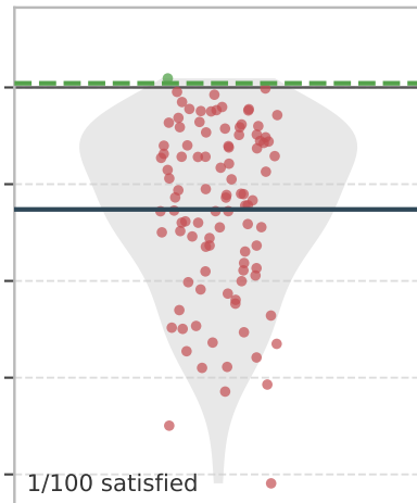
Long Horizon
