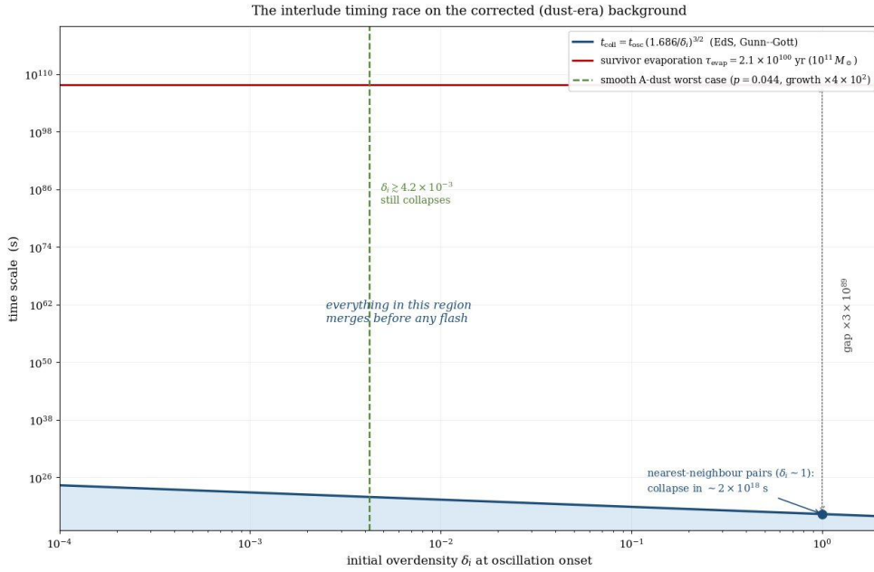
Figure 1: The interlude timing race on the corrected background. Everything in the shaded region merges before any flash. The dashed line marks the smooth-A-dust worst case — now scoped to sub-Jeans scales only; island scales cluster (item F, Fig. 2).
