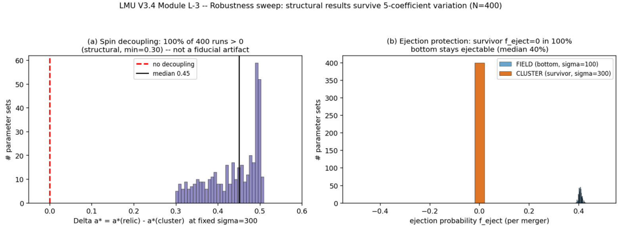
Figure 2: (a) The spin decoupling \Delta a_* across 400 random coefficient sets: it is positive in 100% of them (median 0.45, minimum 0.30), never vanishing. (b) Ejection protection: the cluster survivor stays at f_{\text{eject}} = 0\% in 100% of the space, while the field bottom remains ejectable (median 40%).
