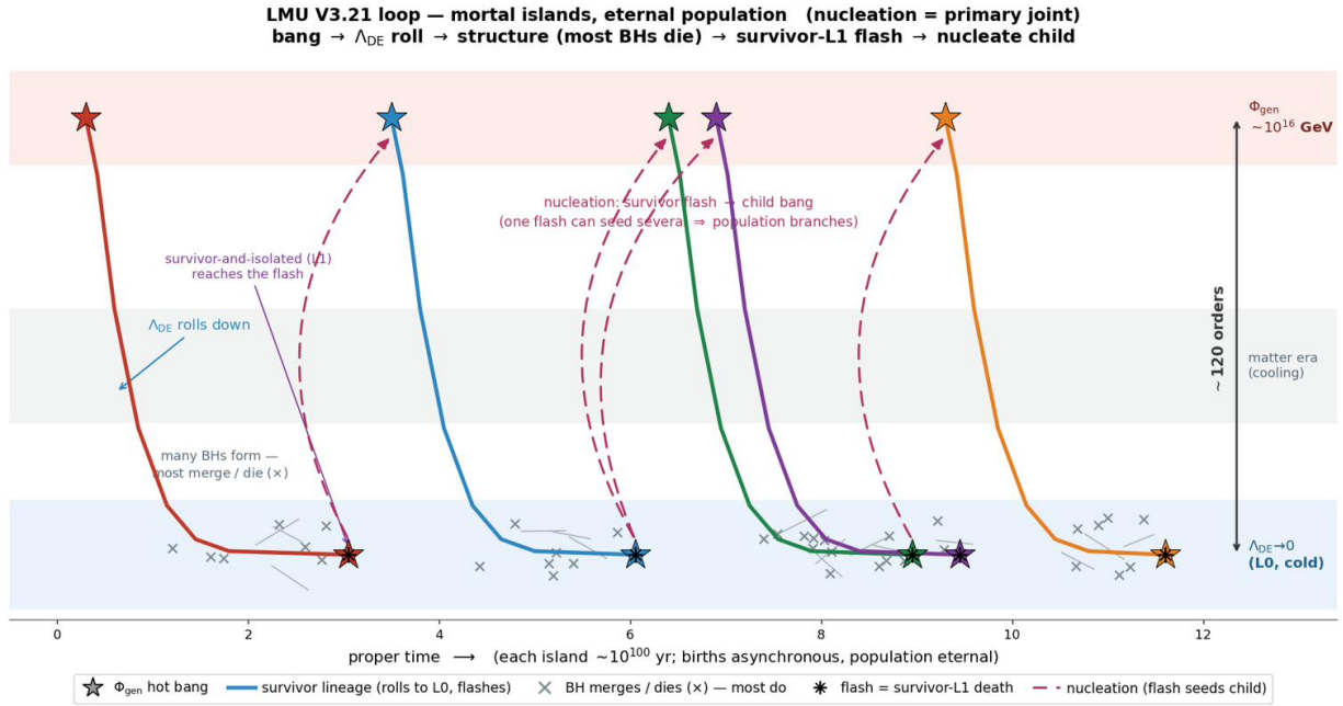
Figure 1: The loop as a cascade, on an energy axis (hot \Phi_{\text{gen}} at top, cold \Lambda_{\text{DE}} \rightarrow 0 at the floor). Each lineage is a hot bang, a roll down to the L0 floor (the A -field thawing toward zero), a long cold span in which most black holes merge or die ( \times ), and the survivor-and-isolated L1’s terminal flash — which nucleates one or more child bangs (B-primary; a flash can seed several). Births are asynchronous and the population is eternal; the right brace marks the \sim 120 orders of magnitude the joint must bridge. Survival, not size: of many holes, only the survivor in each island reaches the flash that seeds the next aeon. [Design] (the composition).
