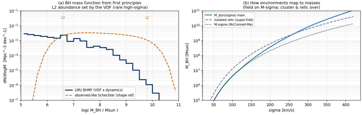
Figure 4: (a) The BH mass function from the environment-weighted dynamics: declining and observed-like, with the L2 end rare because deep hosts are rare ( n_{L3}/n_{L2} \sim \mathcal{O}(10^2) — VDF-parameter and \sigma -bin sensitive (ranging \sim 20 – 500 across reasonable choices), with the top-sparsity following from the dispersion function rather than a tuned merger rate). (b) How environments map to masses: the dynamics produces M – \sigma at low \sigma (field) and rises above it with merger spin-down at high \sigma (cluster), plus the over-massive isolated-relic branch.
