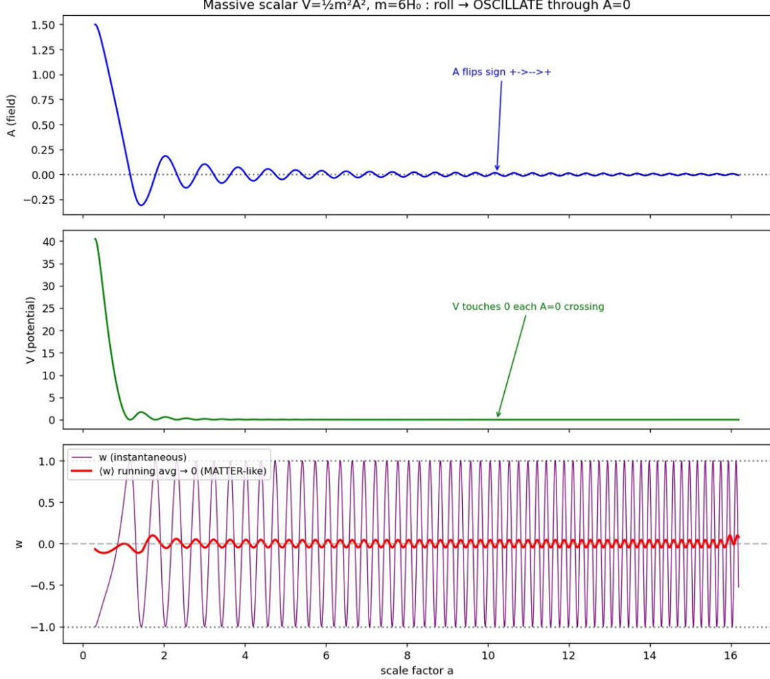
Figure 2: Massive scalar rolling then oscillating: A alternates sign, V touches 0 at each A = 0 crossing, w swings -1 \leftrightarrow +1 , and the running average \langle w \rangle \rightarrow 0 (matter-like).
